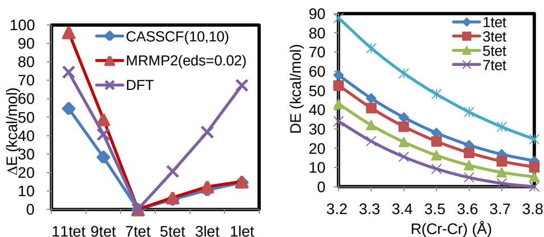
Figure A2-6. PES of \mathbf{MB}_{\text{Cr}} by the CASSCF(10,10) method.
