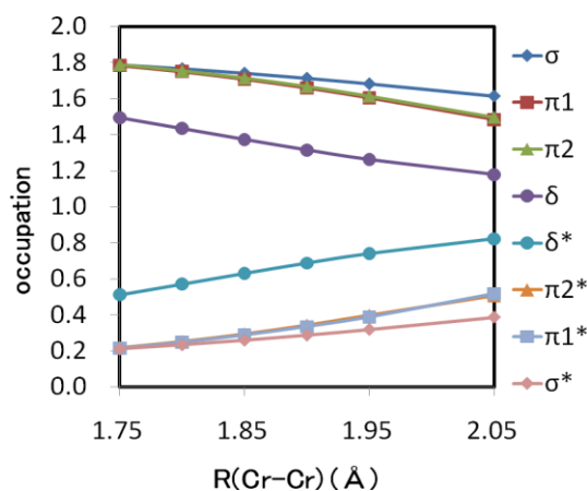
Figure A1-5. The occupation number of [\text{Cr}(\text{R}_1\text{NC}(\text{R}_2)\text{NR}_3)_2]_2 ( \text{R}_1=\text{H} , \text{R}_2=\text{H} , \text{R}_3=\text{H} ) ( M1 )
