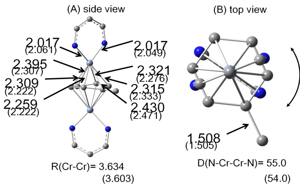
Figure A2-2. Optimized geometry of TB Cr by the DFT(B3LYP) method in septet state under C_1 symmetry. Parentheses represent experimental values. Length in Å and angle in degree.
