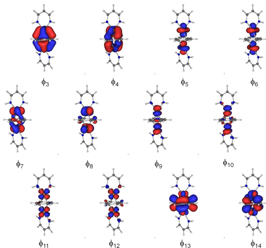
Figure 2-8. CASSCF-optimized MOs of MB Fe in D_2 symmetry.
