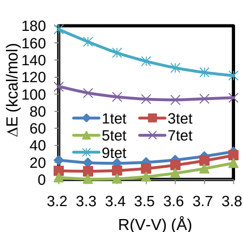
Figure A2-8. PES of MB V by the MRMP2 method using the CASSCF(8,8)- optimized geometries in 1tet to 9tet spin states ..
