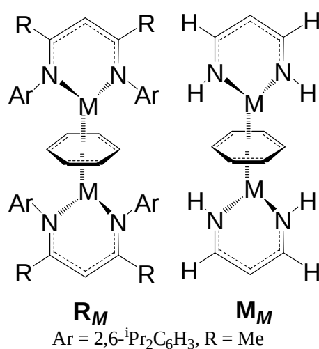
Scheme 3-1. (\mu\text{-}\eta^6:\eta^6\text{-C}_6\text{H}_6)(\text{MDDP})_2 ( R M ) and (\mu\text{-}\eta^6:\eta^6\text{-C}_6\text{H}_6)(\text{MAIP})_2 ( M M ), (M = Y - Tc, DDPH = 2-{4-{(2,6-diisopropylphenyl)imino}pent-2-ene, AIPH = (Z)-1-amino-3-imino-prop-1-ene)
