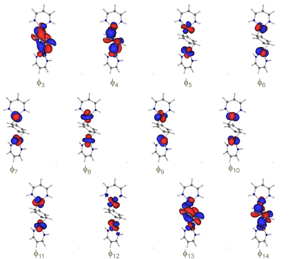
Figure A2-13. The natural orbitals of \mathbf{B}_{\mathbf{Mn}} in the DFT(BP86)-optimized geometry under C_2 symmetry. Only the model part is shown.
