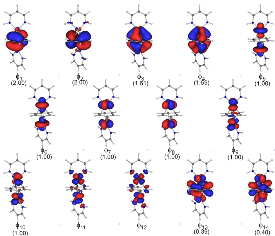
Figure 2-2. CASSCF(10,10)-optimized MOs of MB Cr in D_2 symmetry. Numbers in parentheses represent CASSCF(10,10)-calculated occupation numbers of natural orbitals. a a: We present the occupation numbers of the natural orbitals here, since the natural orbital resembles well the CASSCF-optimized MO.
