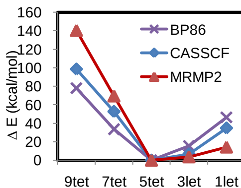
Figure A2-9. Energies (in kcal/mol) of B V relative to the energy of the quintet spin state a
