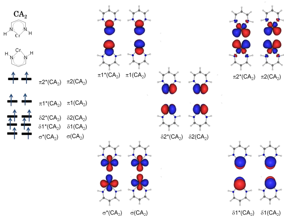
Figure A2-3. Important MOs of Cr(AIP) 2 , CA 2
