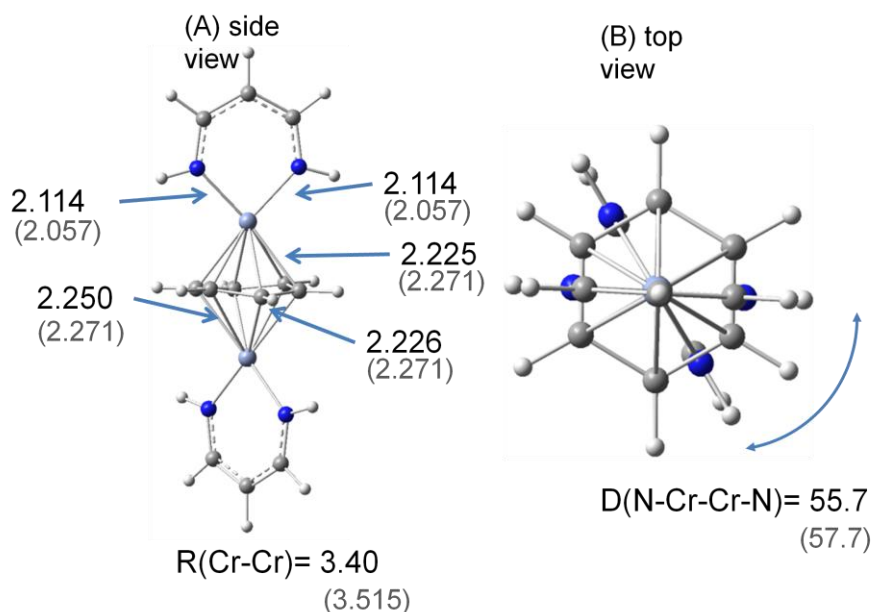
Figure A2-7. Optimized geometry of MB Cr at R(\text{Cr-Cr}) = 3.4 \text{ \AA} by the CASSCF(10,10) method in septet state under D_2 symmetry. Parentheses represent experimental values. Length in \text{\AA} and angle in degree.
