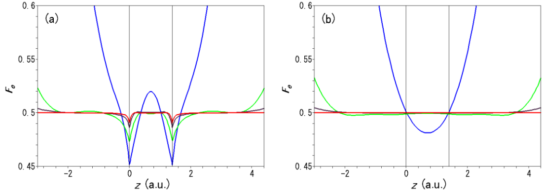
Figure 4-3. (a) Plots of the electron-electron cusp function F_e along the z coordinate that connects two protons lying at z = 0 and z = 1.4011 au at different iteration process of the free ICI calculations using the g_2 function and the initial function \psi_0^{(6)} : Iteration number n = 1 (blue), n = 2 (green), n = 3 (violet) and n = 4 (red). The wave function at n = 4 is our best wave function reported in this paper. (b) Plots of the electron-electron cusp function F_e along the axis lying parallel to the z coordinate that connects two protons lying at z = 0 and z = 1.4011 au at different iteration process of the free ICI calculations using the g_2 function and the initial function \psi_0^{(6)} : Iteration number n = 1 (blue), n = 2 (green), n = 3 (violet) and n = 4 (red). The wave function at n = 4 is our best wave
