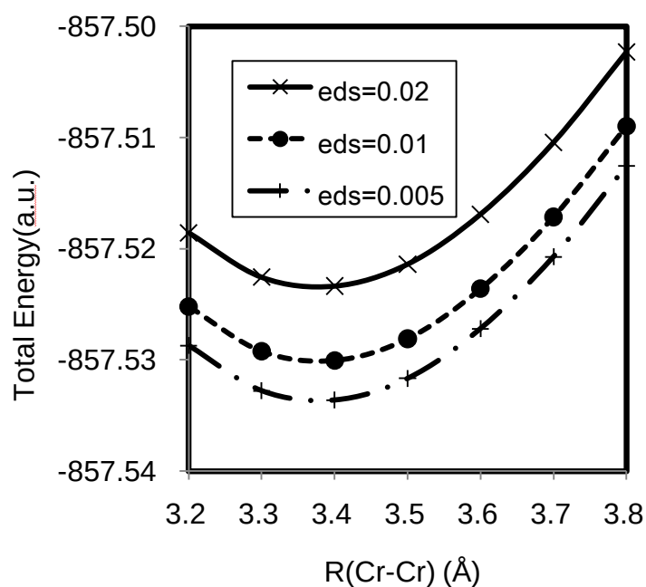
Figure A2-1. Effect of energy denominator shift (EDS) values on the PES of \mathbf{MB}_{\text{Cr}} in the septet spin state calculated by the MRMP2 method a . The equilibrium distances are 3.3749, 3.3831, and 3.3850 Å at EDS=0.02, 0.01, and 0.005, respectively.
