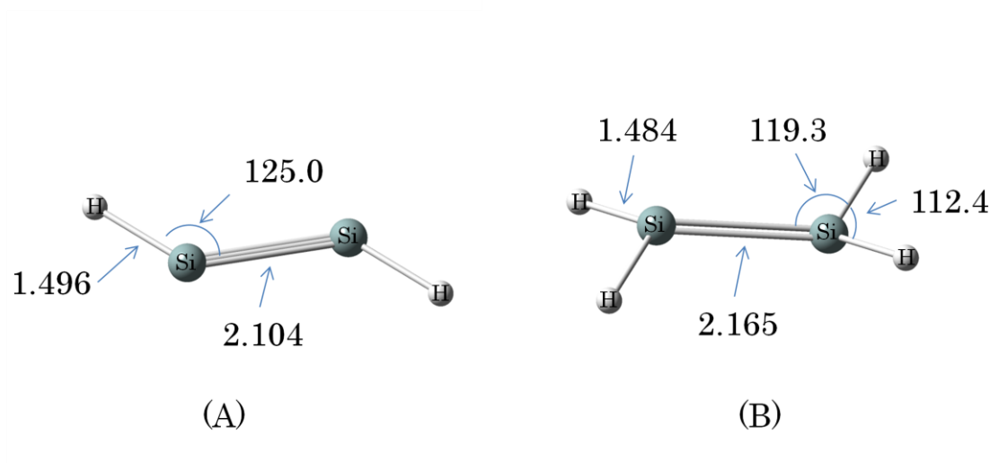
Figure A1-1. DFT-optimized geometries of HSi≡SiH ( S1 ) (A) and H 2 Si=SiH 2 ( S2 ) (B). Length in Å and angle in degree.
