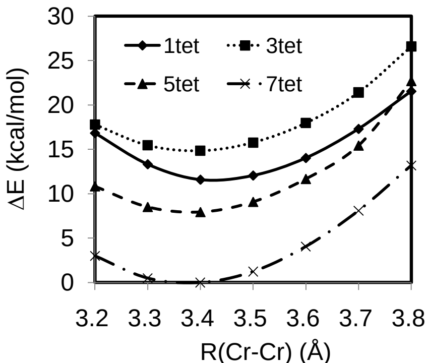
Figure 2-4. Potential energy surface of \mathbf{MB}_{\text{Cr}} calculated by the MRMP2 method. a
