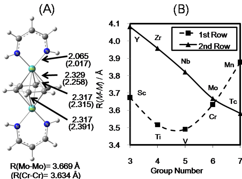
Figure. 3-1 DFT-optimized geometry of \mathbf{M}_M in the most stable spin state. a (A) Important distances (Å) of \mathbf{M}_{Mo} and \mathbf{M}_{Cr} in parentheses (B) Metal-Metal distances of \mathbf{M}_M .
