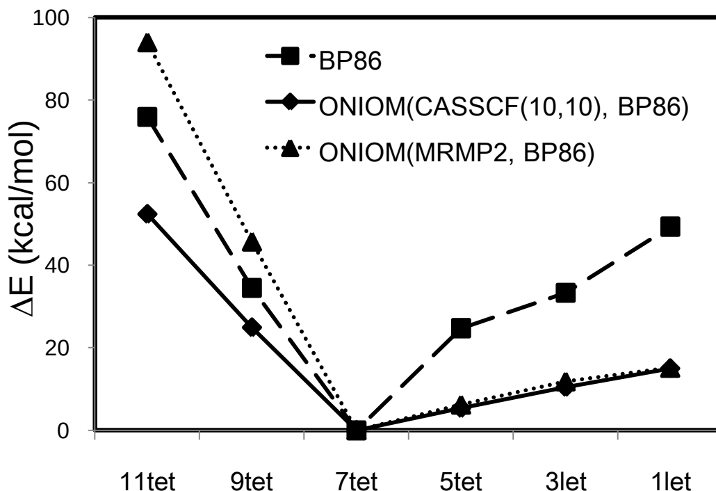
Figure 2-5. Energies of various spin multiplicities of \mathbf{B}_{Cr} relative to that of the 7tet spin state. a
