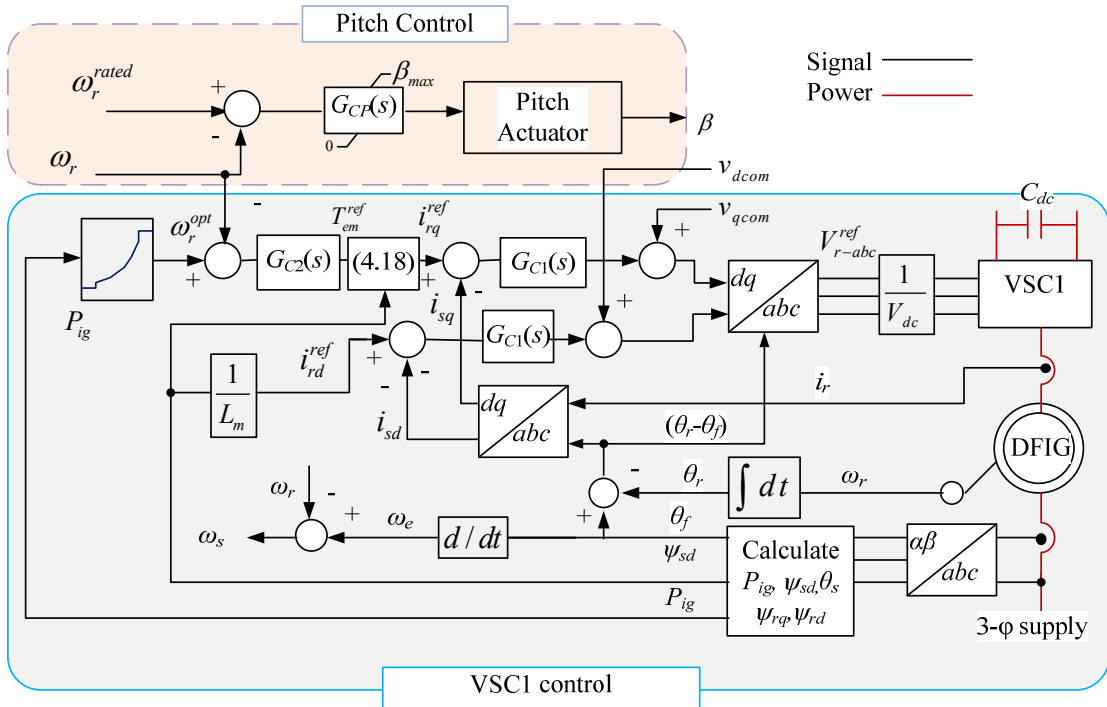
Fig. 4-5 Block diagram of overall control scheme for the DFIG.
