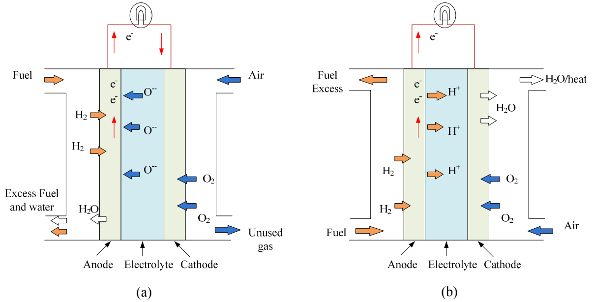
Fig. 2-2 Schematic block diagram of FCs. (a) SOFC (b) PEMFC
