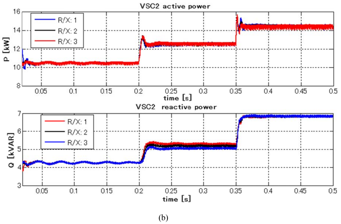
Fig. 6-7 Power flow dynamics of proposed scheme. (a) VSC1', and (b)VSC2.
