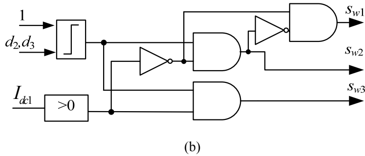
Fig. 3-18 Electrical diagram of the bi-directional dc-dc chopper. (a) Circuit diagram, and (b) switching logic. The variable s_{wi} are the gate signals for the transistor T_i ( i=1,2,3 ).
