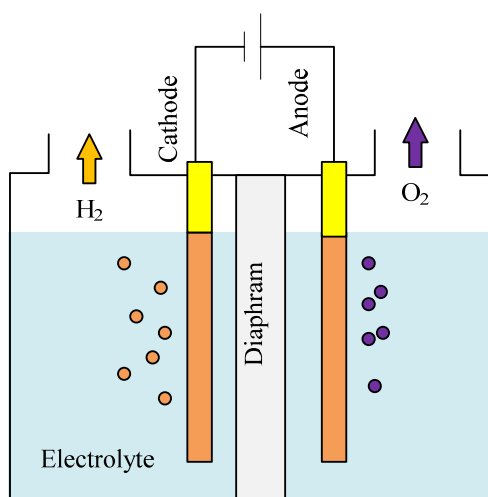
Fig. 2-4 Schemaic diagram of alkaline electrolyzer.
