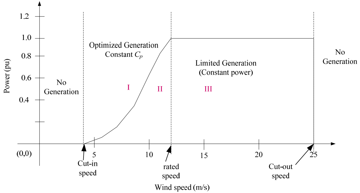
Fig. 3-5 Variable speed pitch controlled wind turbine operation regions.
