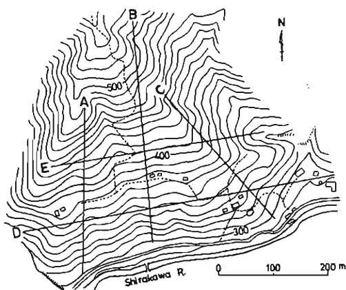
Fig. 17. The map showing the topography of Shirakawa landslide area. A — E: Measuring lines of seismic prospecting.
