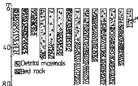
Fig. 4. Geological columnar section at Morito landslide area.
