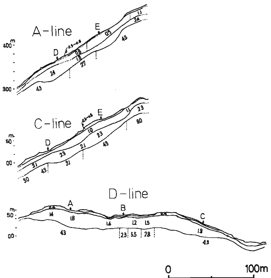
Fig. 18. Underground profile by seismic prospecting at Shirakawa landslide area. Measuring lines are shown in Fig. 15. (after Tokushima Pref., 1972).
