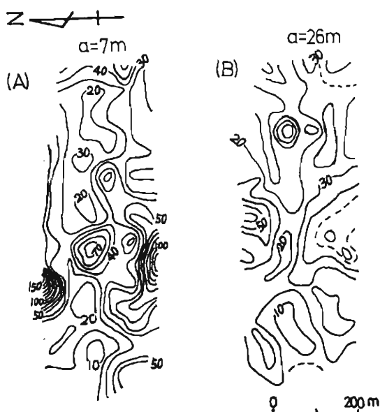
Fig. 10. The Distribution map of apparent resistivity values at Kuraishi landslide area. The map showing the distribution of apparent resistivity values of seven and twenty six meter in depth.
