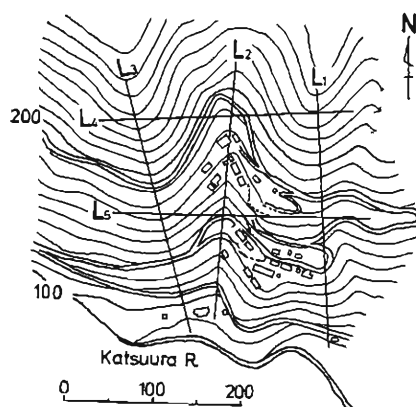
Fig. 11. The map showing the topography of Hiura (Iitani-cho) landslide area L_1 - L_5 : Measuring lines of seismic prospecting.
