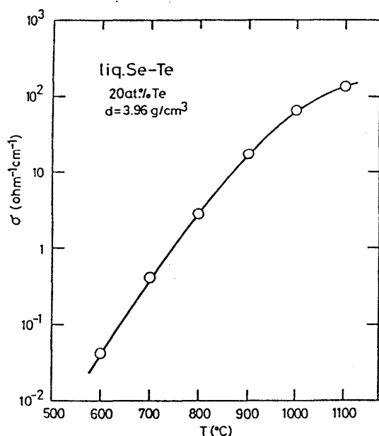
Figure 9. Temperature variations of the electrical conductivity \sigma for liquid Se-Te mixture with 20 at.% Te on the isochore curve with d=3.96 g/cm 3 .
