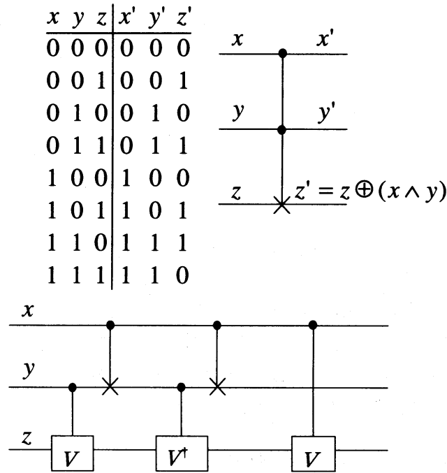
C 2 -NOT(controlled-controlled NOT)
