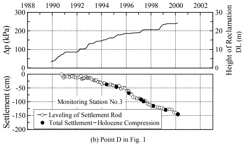
Fig. 5 Measured time-settlement relations at Yumeshima Reclaimed Island with differential settlement gauges
