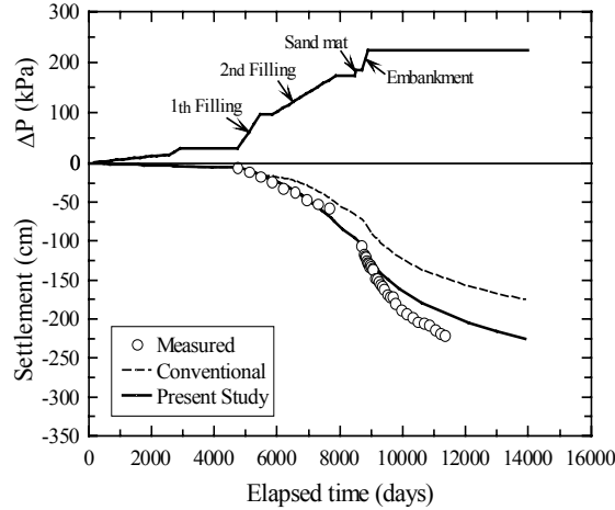
Fig. 17 Comparison of advance in total settlement for Pleistocene clay deposits
