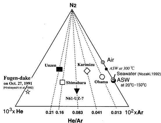
Fig. 5 Relative He, Ar and N 2 contents of gases from boiling spring, hot spring, mineral spring, fumaroles and geothermal well together with those of potential end-member components: air, air-saturated water (ASW), seawater-dissolved gas (Nozaki, 1992) and magmatic gas (volcanic gas from Fugen-dake; Hirabayashi et al., 1992). Symbols correspond to those in Fig.1.
