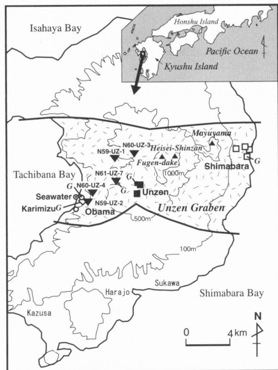
Fig. 1 Location map of hot springs (Obama, Unzen and Shimabara) and geothermal wells in Unzen Graben of the Shimabara Peninsula, Kyushu, Japan. Data sources of this study are from hot springs (○: Obama, ■: Unzen, □: Shimabara), mineral spring (◇: Karimizu) and geothermal wells (▼). G with symbols indicates that geochemical gas data used in this study are taken from these sites (■G: fumarolic gas from Unzen, ○G: steam of boiling spring from Obama, ▼G: separated-steam of thermal water from geothermal well, ◇G: bubble gas of mineral spring from Karimizu, □G: bubble gas of hot spring from Shimabara). Symbol ● indicates sampling site of reference seawater used in this study.
