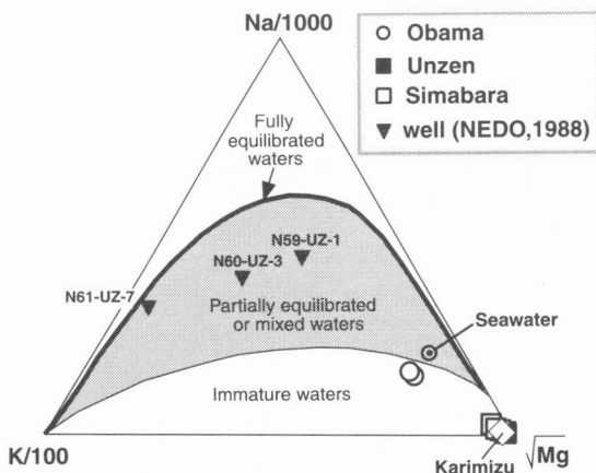
Fig. 3 Ternary plot used to recognize equilibrated waters for waters from hot springs, mineral spring, geothermal wells and seawater from Tachibana Bay. Symbols correspond to those in Fig. 1.
