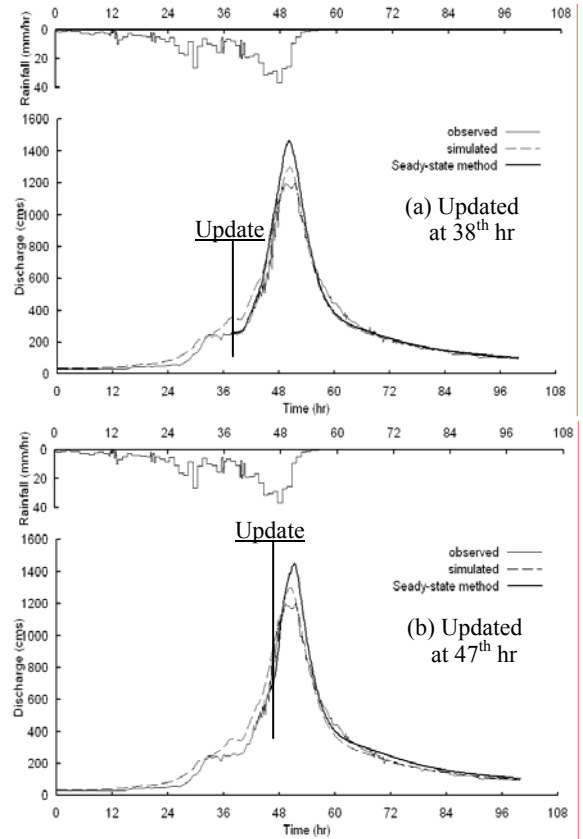
Fig. 4 Update results from steady - state method (Event1).
