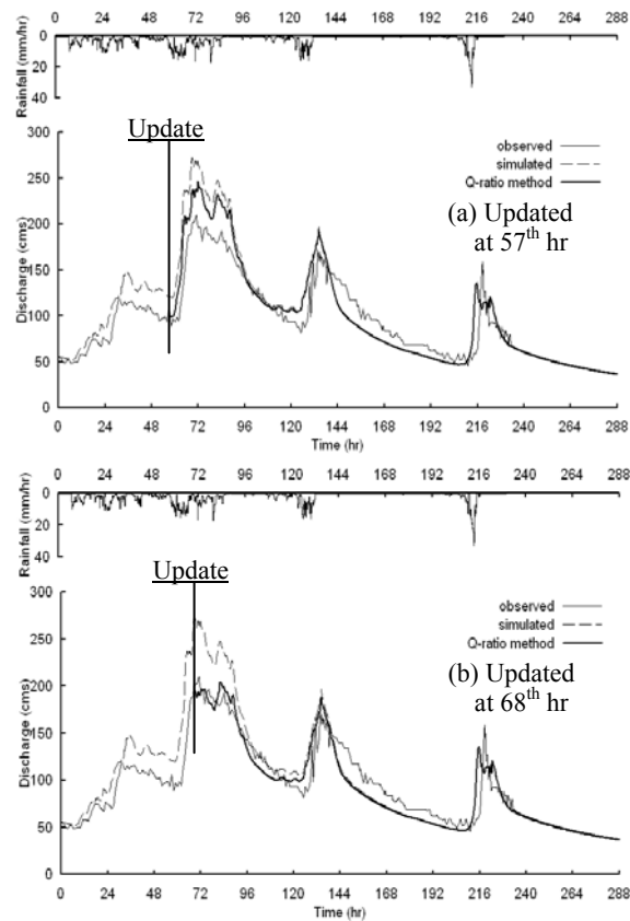
Fig. 12 Update results from Q-Ratio method (Event2).
