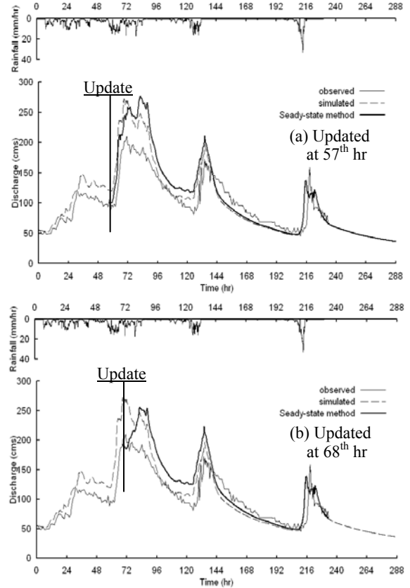
Fig. 5 Update results from steady-state method (Event2).
