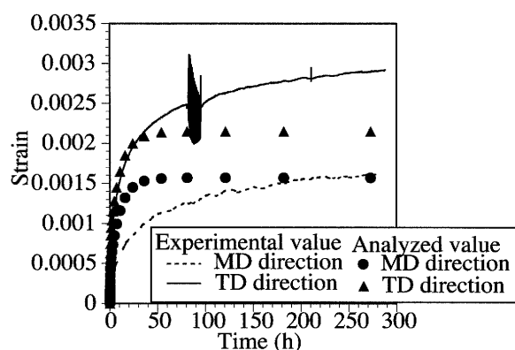
Fig. 13 Measured and analyzed hygroscopic strain of the polarizing plate at 40°C and 60% RH
