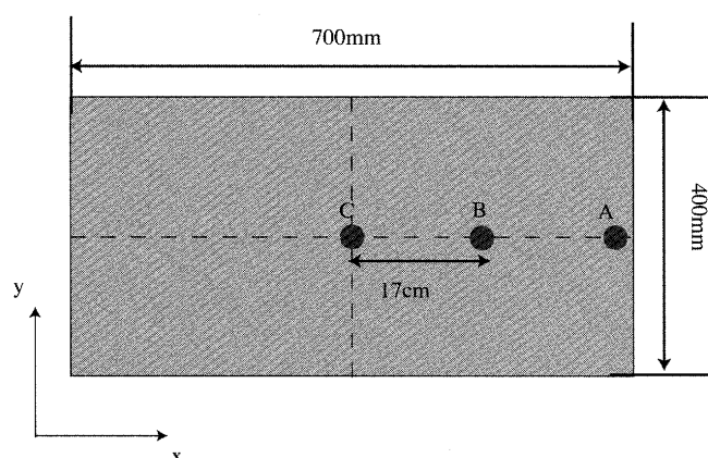
Fig. 14 Locations of strain gauges on an LCD panel
