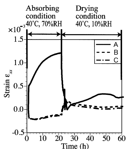
Fig. 15 Measured hygro-strain on an upper surface
