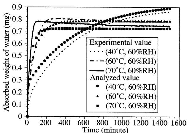
Fig. 5 Measured and analyzed absorbed weight of water in polarizer
