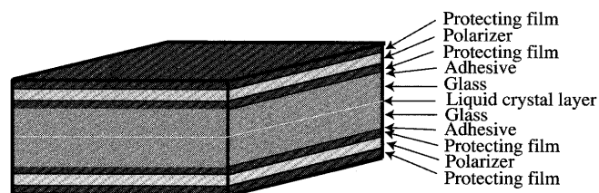
Fig. 1 Structure of an LCD Panel (the MD directions of the upper and lower polarizer sheets are orthogonal)
