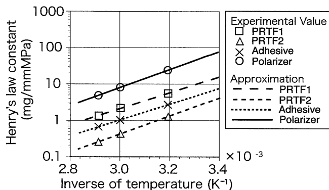
Fig. 6 Arrhenius plot of Henry's law constant
