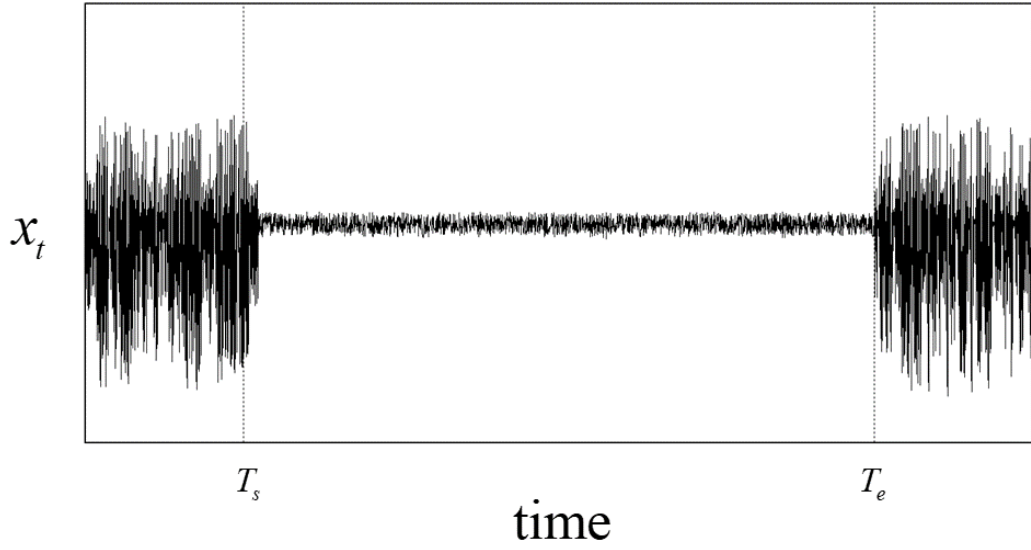
Figure 13: Time series. The OGY method succeeds in stabilizing the system subjected to external shocks. \sigma = 0.05 .
