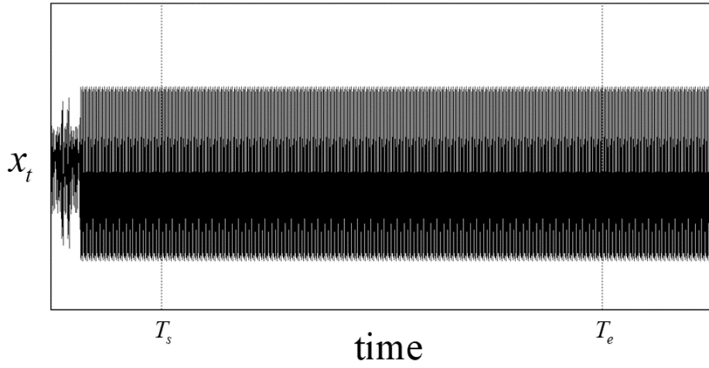
Figure 8: Time series. The OGY method fails to stabilize the system. A = 2 , \alpha = 1/2 , \beta = 7 , s = 0.1 , and \varepsilon = 0.1 .
