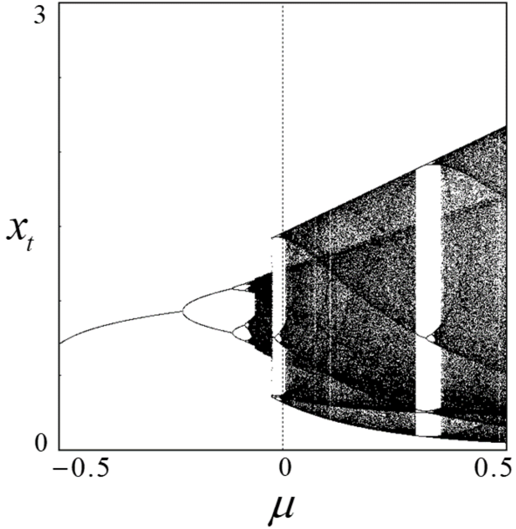
Figure 7: Bifurcation diagram with respect to \mu . A = 2 , \alpha = 1/2 , \beta = 7 , and s = 0.1 .
