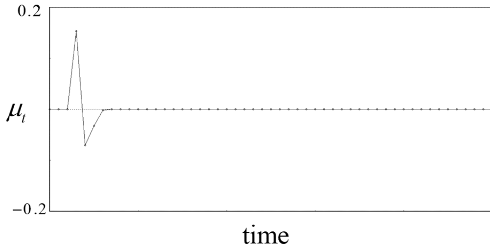
Figure 5: The values of \mu_t stick to zero by 10 steps from the start of control. A = 2 , \alpha = 1/2 , \beta = 8 , s = 0.1 , and \varepsilon = 0.1 . t \in [500, 550] .
