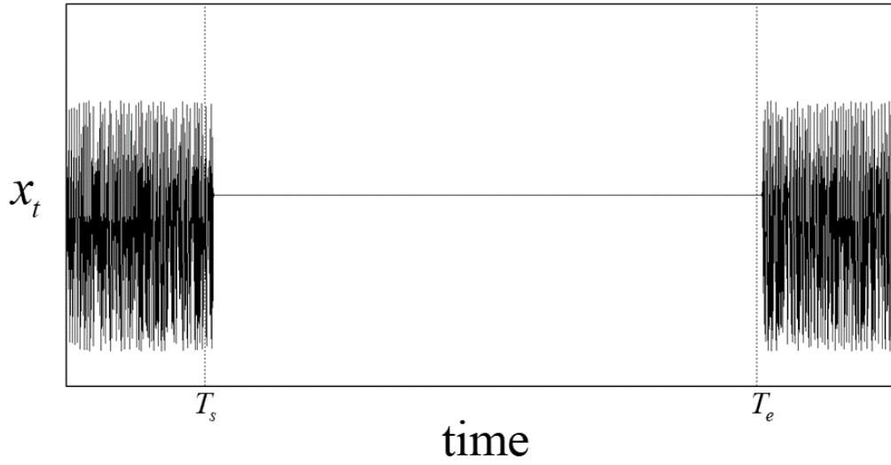
Figure 4: Controlled chaotic time series. It takes some time for the chaotic trajectory to enter the vicinity of the target. As soon as the control is aborted, chaotic behavior reappears. A = 2, \alpha = 1/2, \beta = 8, s = 0.1 , and \varepsilon = 0.1 . t \in [0, 3 \times 10^3] . Control starts at T_s = 500 and stops at T_e = 2,500 .
