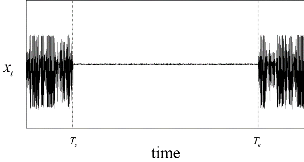
Figure 12: Time series. The OGY method succeeds in stabilizing the system subjected to external shocks. \sigma = 0.01 .
