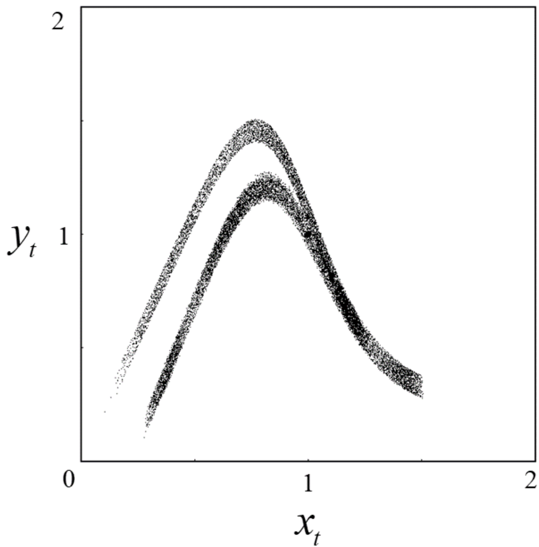
Figure 10: Noisy chaotic “attractor”. The influence of stochastic perturbations reveals the hidden chaotic structure. \sigma = 0.05 .
