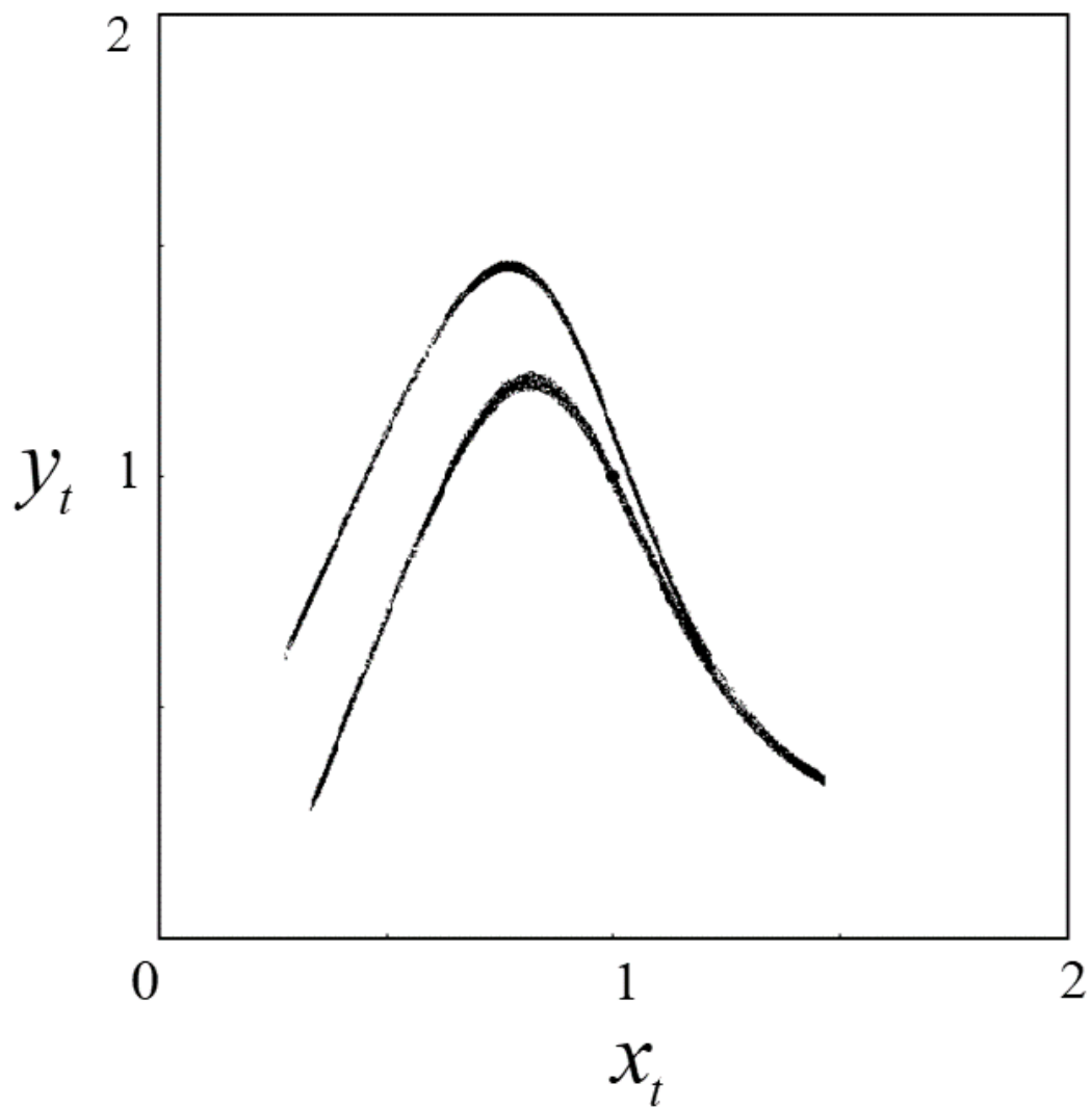
Figure 9: Noisy chaotic “attractor”. The influence of stochastic perturbations reveals the hidden chaotic structure. \sigma = 0.01 .
