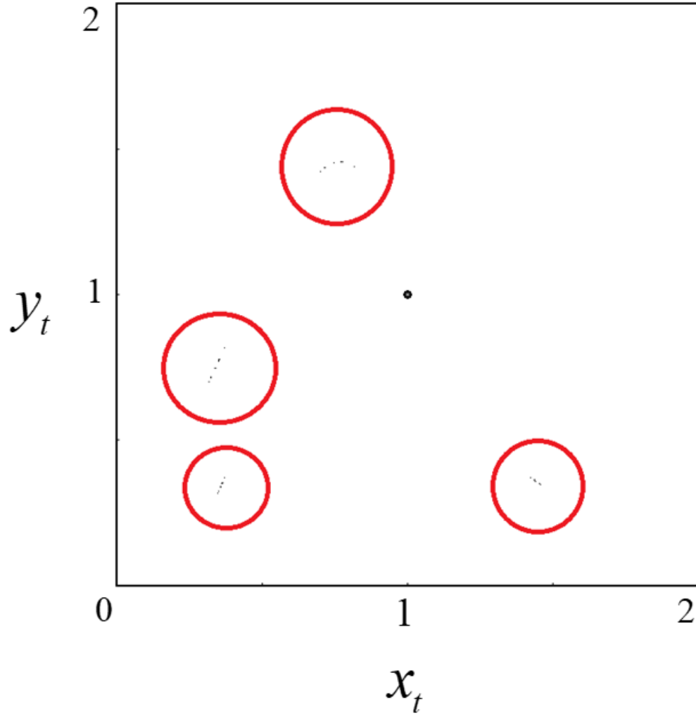
Figure 6: The target steady state is far from the attractor. The attractor is contained in the red circles. The transients are omitted. A = 2, \alpha = 1/2, \beta = 7, s = 0.1 , and \mu = 0 .
