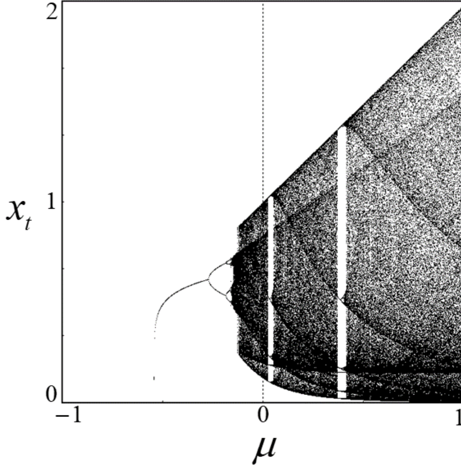
Figure 2: Bifurcation diagram. The parameter \mu , the growth rate of money, moves from -1 to 1 A = 2, \alpha = 1/2, \beta = 8 , and, s = 0.1 . Money loses value if \mu falls below a certain value. For some range of the value of \mu , which is negative, the golden rule steady state is an attractor, whereas chaotic fluctuations are observed for a much larger set of \mu values.
