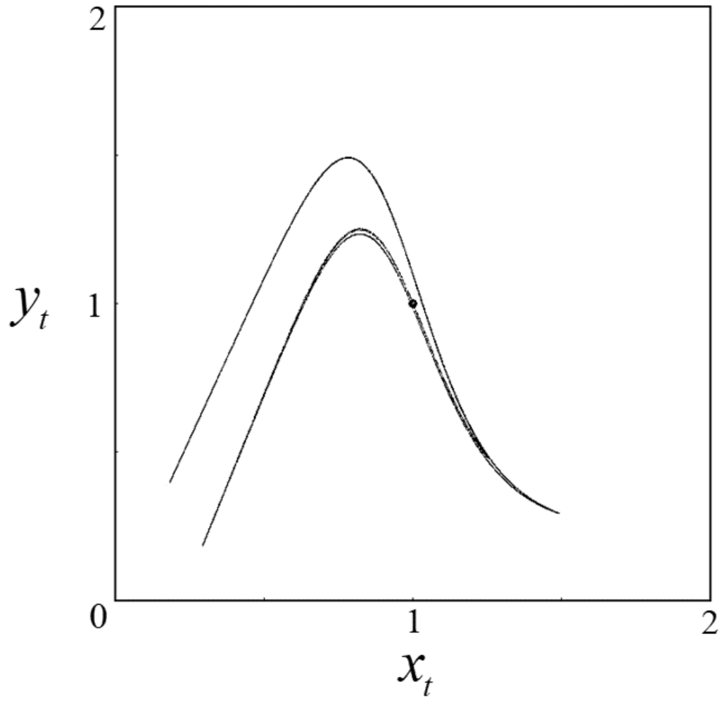
Figure 1: Chaotic attractor on the plane. The golden rule steady state (1, 1) is highlighted. The transients are omitted. A = 2 , \alpha = 1/2 , \beta = 8 , s = 0.1 , and \mu = 0 .
