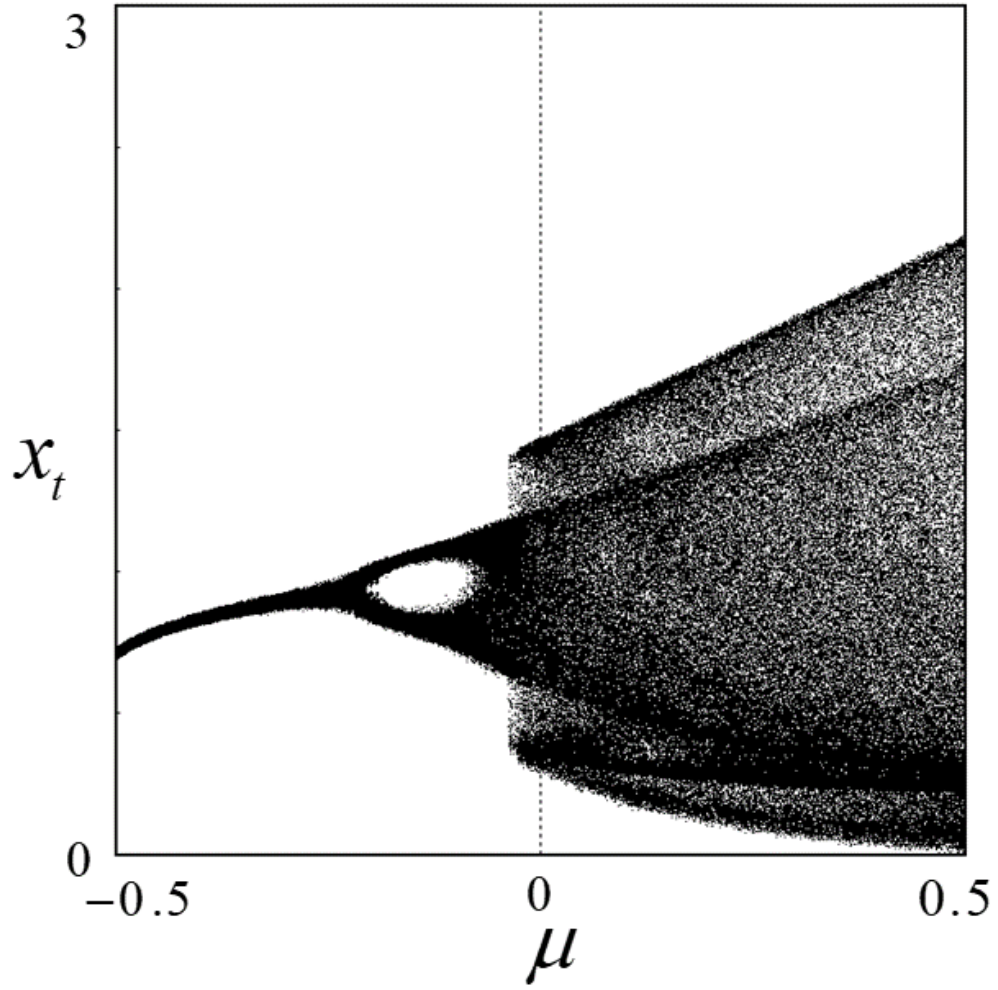
Figure 11: Compared with Figure 7, most of the windows have disappeared due to small external shocks. \sigma = 0.01 .
