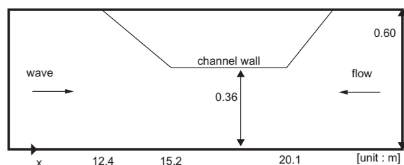
Fig. 2 Experimental setup (Chawla and Kirby, 1998)
