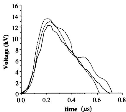
Fig. 8. Calculated wave shapes of the tower top voltage by two different propagation velocities. (——measured, ———light velocity, .....80% of the light velocity)
