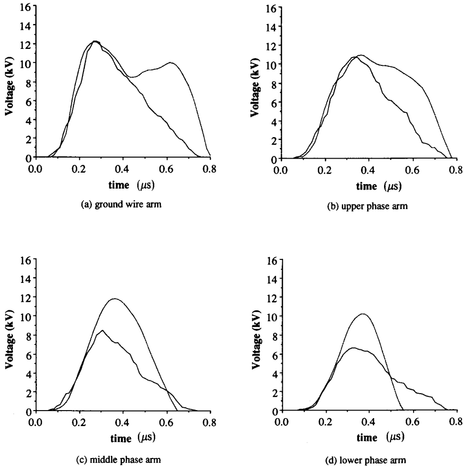
Fig. 6. Comparison between measured and calculated voltage wave shapes at various points on the tower.
