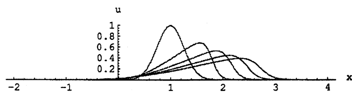
图 6.3: FDM( \Delta x = 2^{-4} , \Delta t = 2^{-8} )
