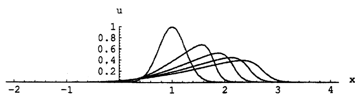
图 6.1: SCM( \Delta x = 2^{-4} , \Delta t = 2^{-8} )
