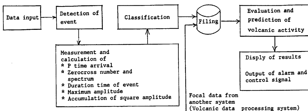
Fig. 3. General flow of the data processing.
