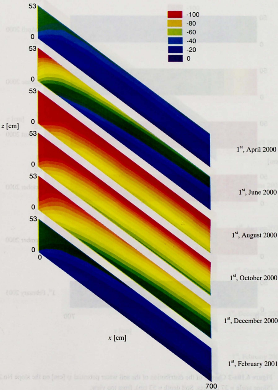
Figure 6.10a-1 Change of the distribution of the soil water potential \psi [cm] on the slope No.2 (Slope angle = 37 degrees, Soil depth = 53 cm), from side view.
