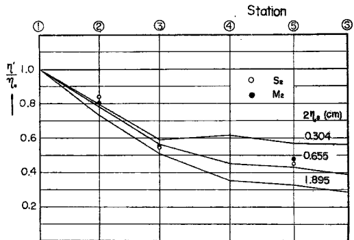
Fig. 9 Ratio of amplitude for semi-diurnal tide
