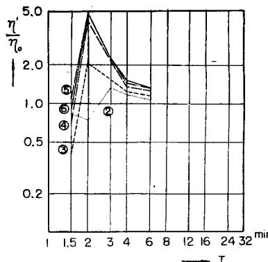
Fig. 18 Experimental frequency response (dredged state with small reservoir)
