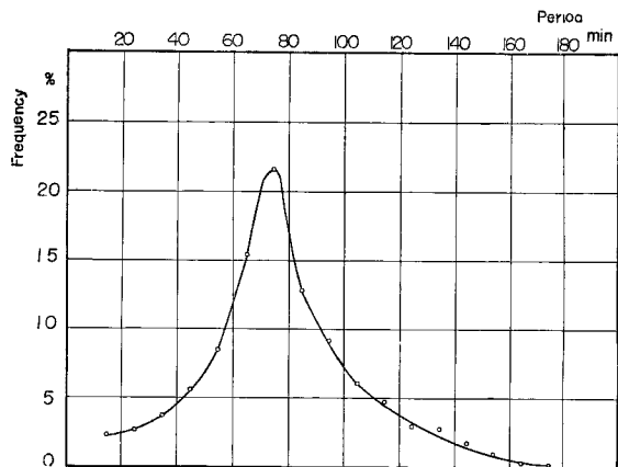
Fig. 3 Frequency distribution of long period waves at Mihonoseki tidal station (prototype)
