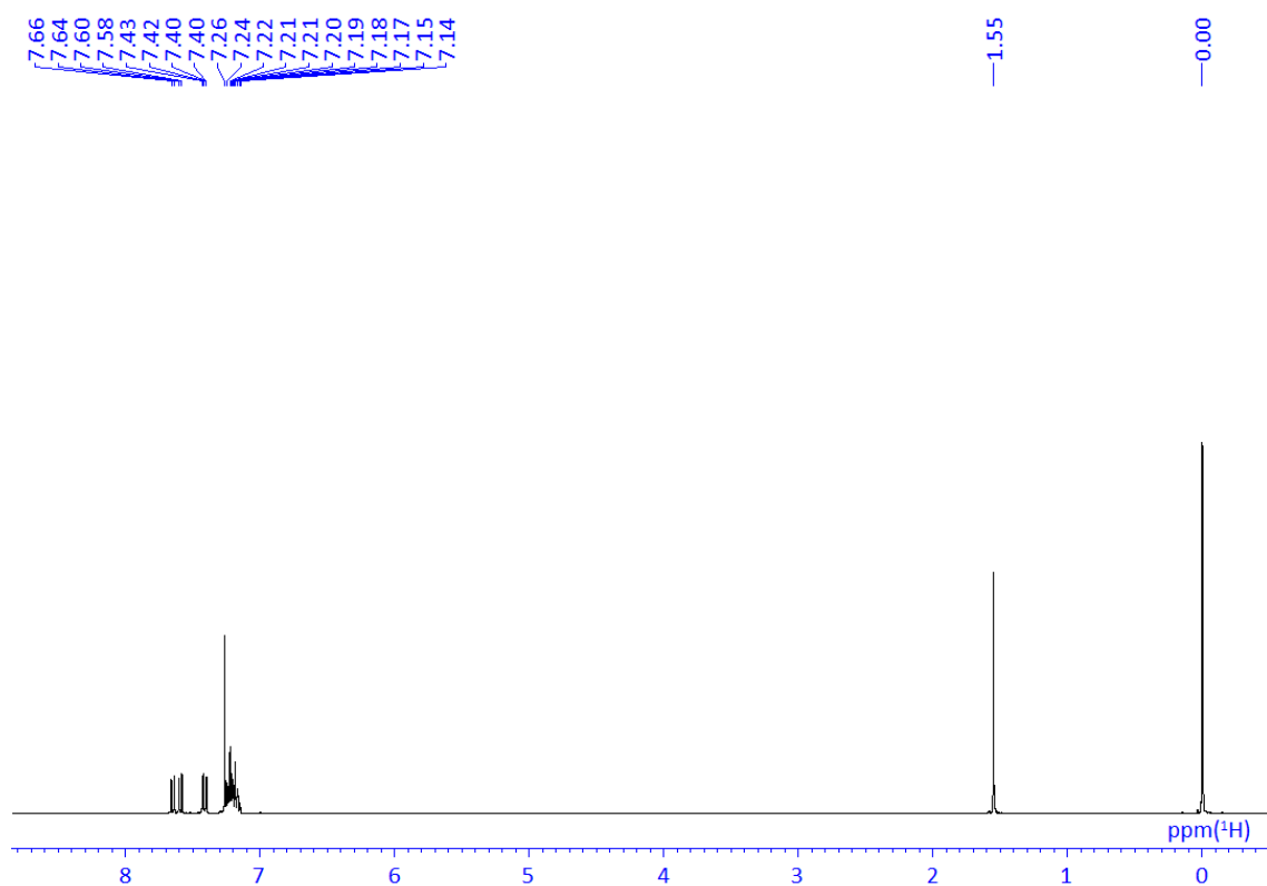
Chart 7. 1 H NMR spectrum of BAz-Ph in CDCl 3 .
