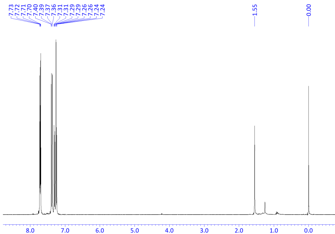
Chart 1. 1 H NMR spectrum of BAz-C6F5 in CDCl 3 .
