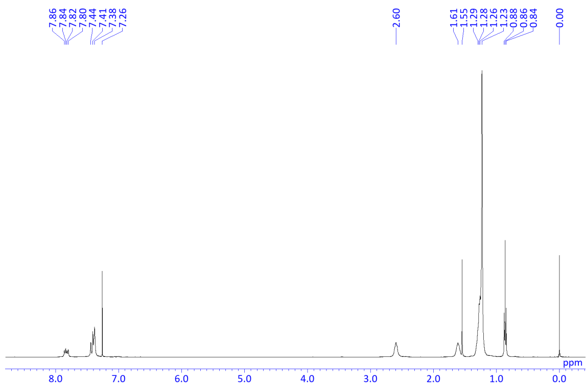
Chart 4. 1 H NMR spectrum of P-BAz-C6F5 in CDCl 3 .
