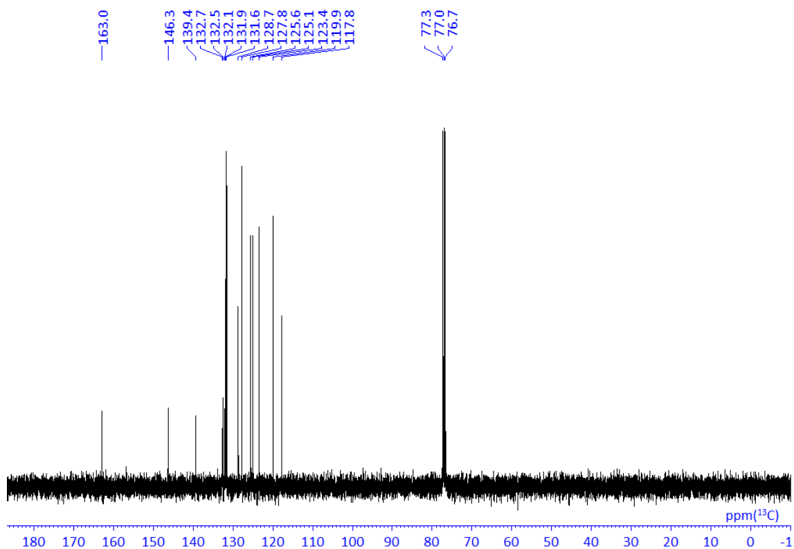
Chart 8. 13 C NMR spectrum of BAz-Ph in CDCl 3 .
