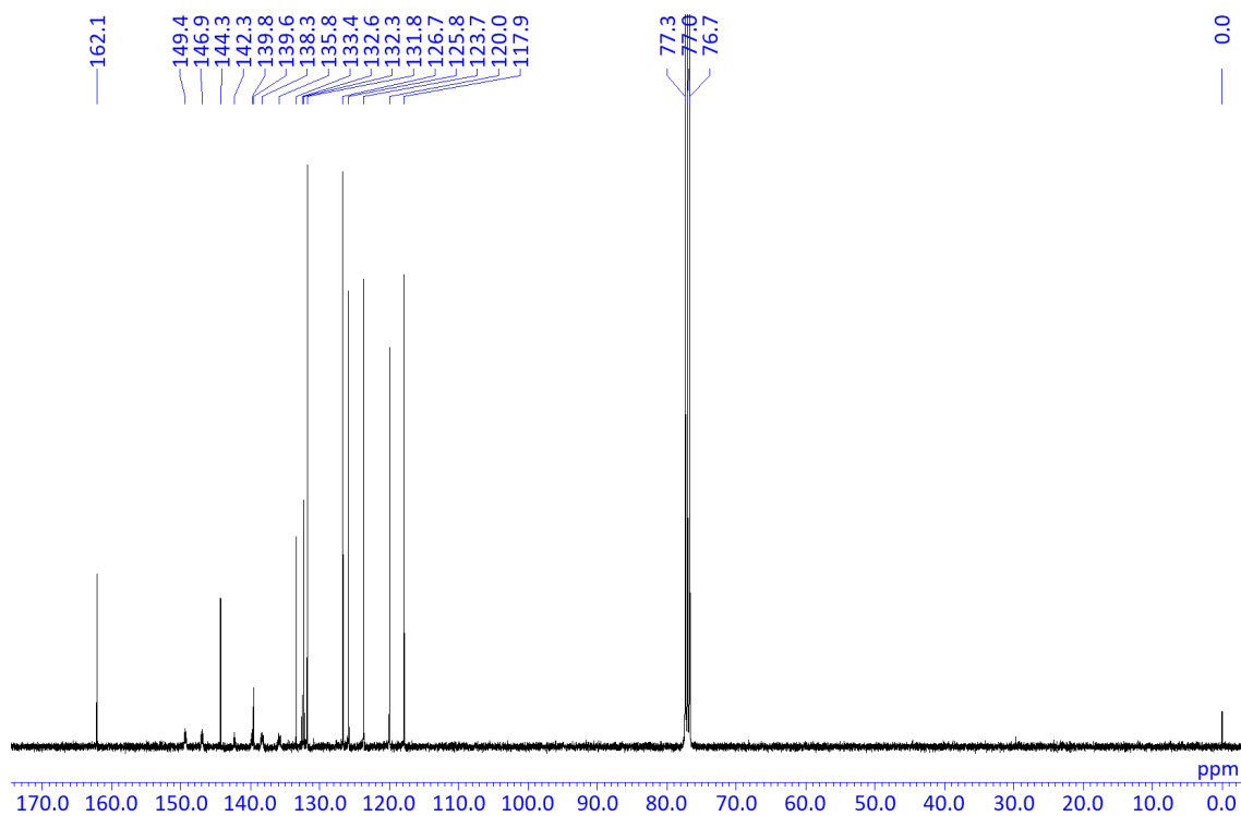
Chart 2. 13 C NMR spectrum of BAz-C6F5 in CDCl 3 .
