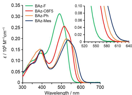
Figure 1. UV-vis absorption spectra of the BAz complexes in toluene ( 1.0 \times 10^{-5} M).
