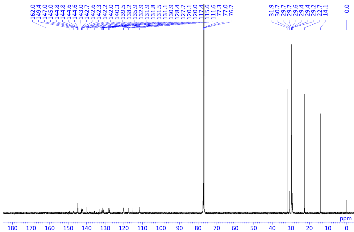
Chart 5. 13 C NMR spectrum of P-BAz-C6F5 in CDCl 3 .
