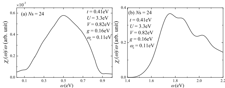
Fig. 1. Optical conductivity in a Hubbard-Holstein chain with 24 sites, taken from Ref. [3]. (a) Phonon-assisted spin excitation, and (b) Mott-gap excitation. The broadening factor \sigma = 0.04 eV. Parameter values are shown in the panels.
