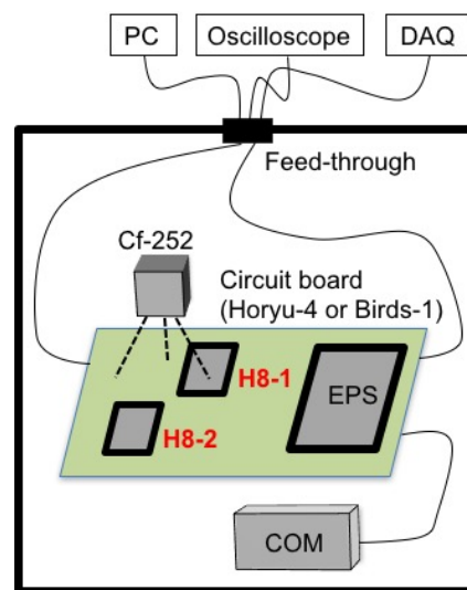
Fig. 1 Test setup of Horyu-4 and BIRDS-1
