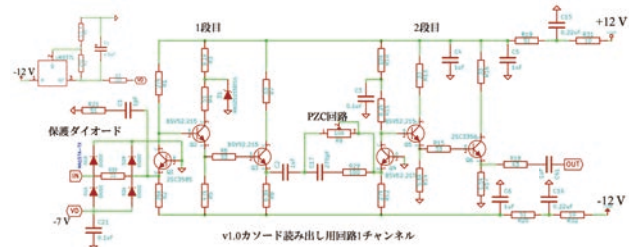
Fig. 2. Circuit diagram of the amplifier
