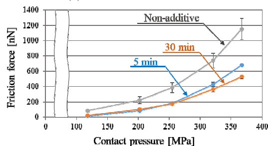
(b) With disodium sebacate
