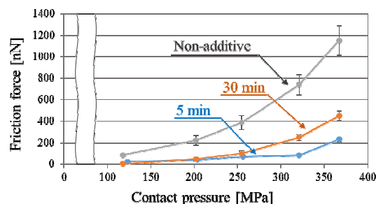
(a) With sodium decanoate
