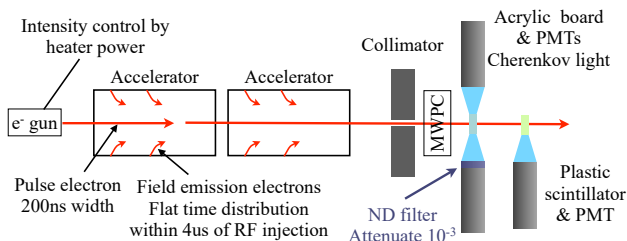
Fig. 1. Experimental setup
