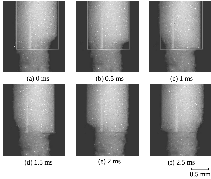
Fig. 2. Snapshots of the powder flow at the end of the vibrating capillary made of glass (Silica particles: MMD = 30.4 \mu\text{m} , vibration frequency: f = 330 \text{ Hz} , vibration amplitude: a = 130 \mu\text{m} )
