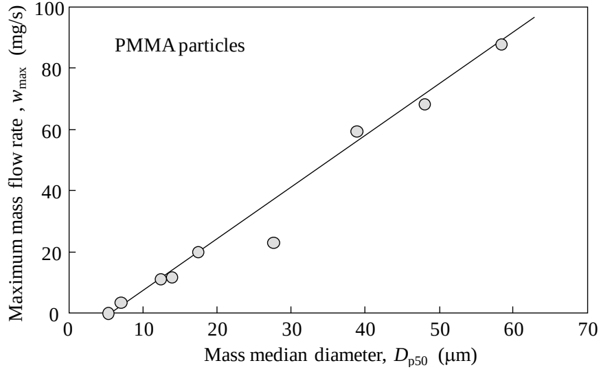
Fig. 8 Relationship between maximum mass flow rate and mass median diameter
