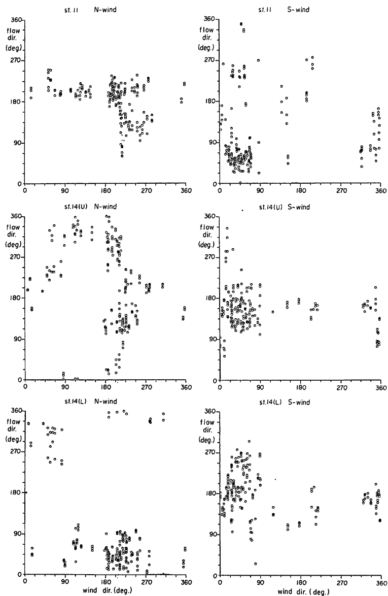
Fig. 11 Relationships between wind and flow direction ( 0^\circ , northward; 90^\circ , eastward) under north and south wind conditions
