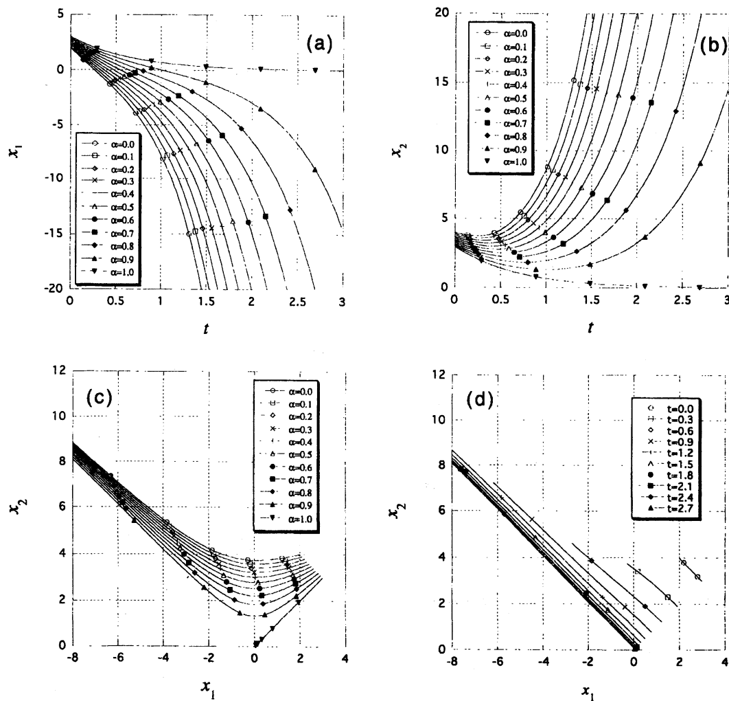
Fig. 6. Computed results for Case I.
