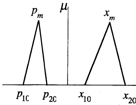
Fig. 5. Membership functions \mu in the numerical calculation.
