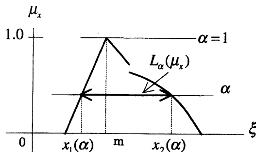
Fig. 1. Fuzzy number and its parametric representation with endpoints of \alpha -cut set.
