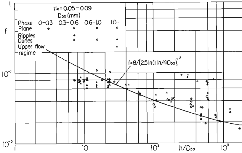
Fig. 2 Relationship between f and h/D_{50} in range 0.05 \leq \tau_* \leq 0.09
