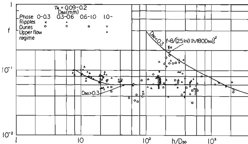
Fig. 3 Relationship between f and h/D_{50} in range 0.09 \leq \tau_* \leq 0.2
