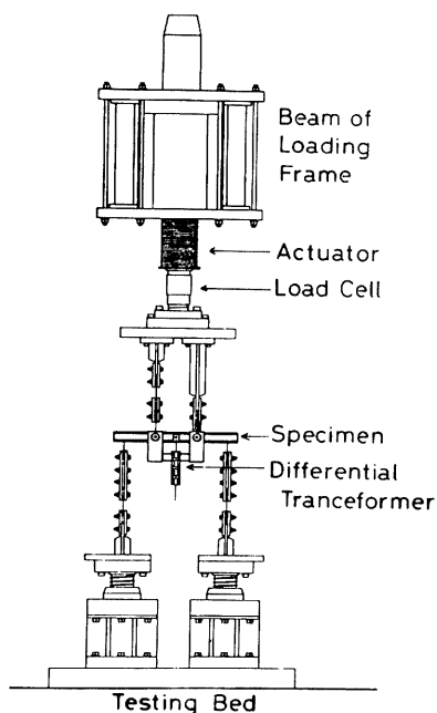
Fig. 13. Testing System.
