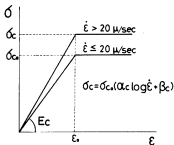
Fig. 25. Stress-Strain Curve for Concrete.
