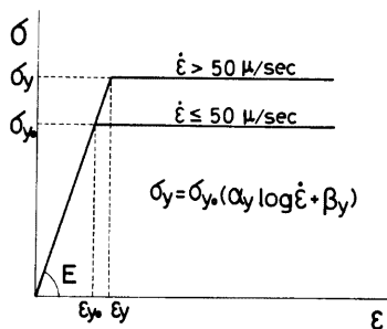
Fig. 23. Stress-Strain Curve for Steel.
