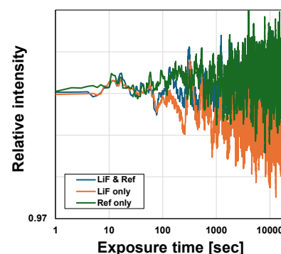
Fig.2 Accelerated degradation test of SOF detector components.
