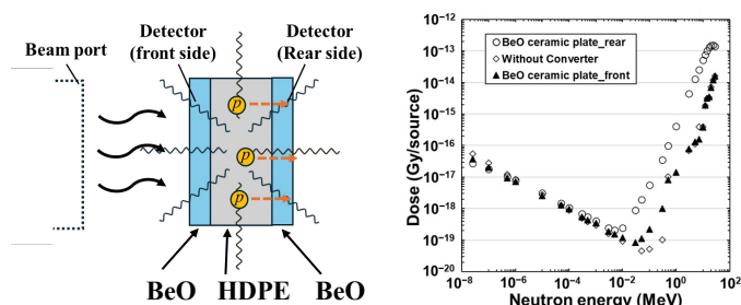
Fig. Schematic configuration of the proposed detector and calculated neutron energy response.
