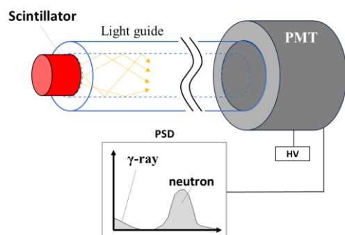
Fig. 1. Schematic layout of neutron detector
