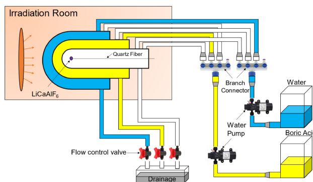
Fig. 1. Outline of a prototype CHARMS.
