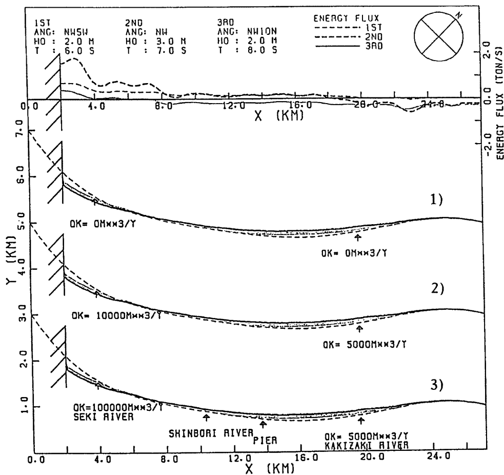
(a) Upper: wave energy flux, 2nd: no sediment supply from rivers, 3rd: 10,000 m³/yr from Seki river and 5,000 m³/yr from Kakizaki river, bottom: 100,000 m³/yr from Seki river and 5,000 m³/yr from river.
