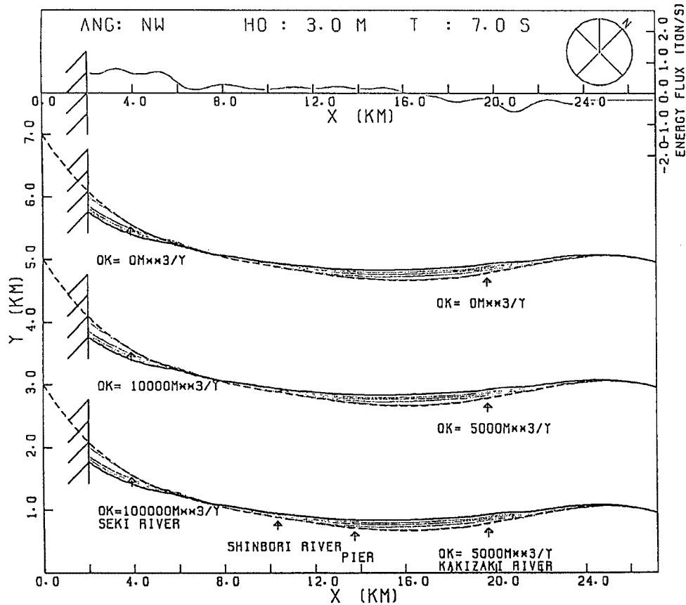
Fig. 5.7. Computed shoreline changes in the period of 1910-1960 assuming the 2nd representative wave condition.
