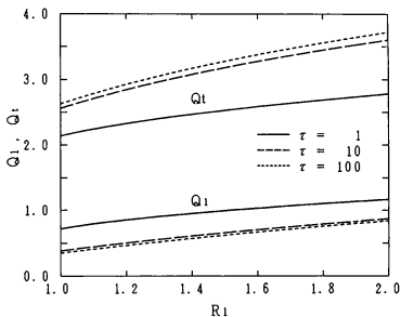
FIG. 2.7. The normalized ion energy flux Q_i and the normalized total energy flux Q_t = Q_i + Q_{ie} at the plasma-sheath boundary as a function of the mirror ratio R_1 , where Q_{ie} is the normalized electron energy flux.
