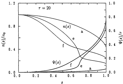
FIG. 5.5. Profiles of the normalized presheath potential (thick lines) and the particle density (thin lines) for n_{A0}/n_0 = 0.10, 0.28 , and 0.50 , where the spatial profile of the particle source is chosen as h(s) = n(s)/n_0 . The wall is located at s = 1 . Symbols a , e , and f represent results for the points in Fig. 5.2.
