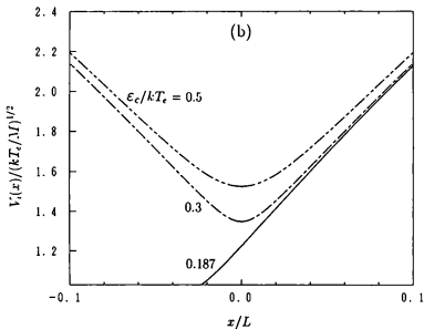
FIG. 4.5(b). Profiles of the ion drift velocity of the hot-ion plasma near the magnetic throat of the model field. The values of the cutoff energy \epsilon_c are \epsilon_c/kT_e = 0.187 , 0.3 , and 0.5 .
