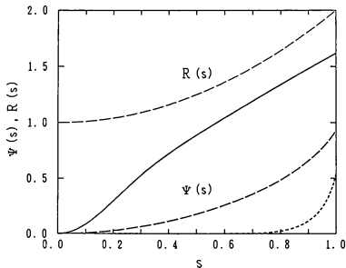
FIG. 3.7. The normalized potential profile for the partial source with the spatial distributions h(s) = \exp(-25s^2) (—), h(s) = 1 (---), and h(s) = \exp(-25(1-s)^2) (-·-·-·-). The magnetic mirror ratio profile is chosen as R(s) = 1 + s^2 .
