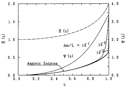
FIG. 2.8. The profile of the normalized potential \Psi(s) for an ion source with \tau=1 for various values of \lambda_{D0}/L , where the model field R(\Psi)=\exp(\alpha\Psi) with \alpha=0.536 is described by the use of the analytic solution, \Psi , (heavy line) of the plasma equation.
