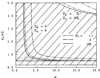
FIG. 4.3. Domain in \alpha - \epsilon_c space where monotonically varying continuous potential can be formed in the cold-ion plasma with T_{i||} = 0 and T_{i\perp} = 0 , and in the hot-ion plasma with T_{i||} = T_e and T_{i\perp} = 10T_e flowing through expanding magnetic field with various mirror ratios at the wall. Here \alpha is the reducing parameter of the model electron distribution function given by Eq. (4.8) and \epsilon_c is the cutoff energy of the model ion distribution function given by Eq. (4.7).
