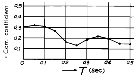
Fig. 12 Space correlation of two measurement points on eaves and roof.
