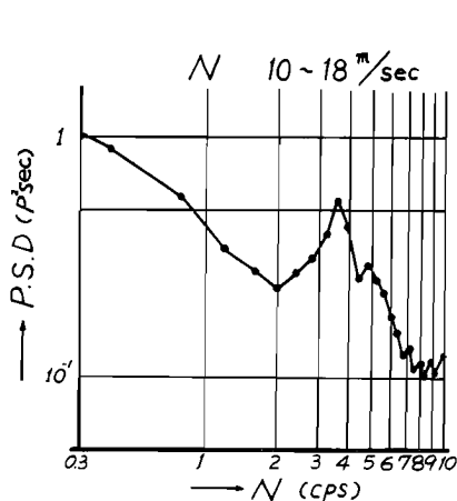
Fig. 2 Spectrum of the wind pressure fluctuation on eaves of House A.
