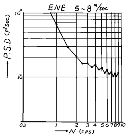
Fig. 11 Spectrum of the wind pressure fluctuation by free-direction pressure gage nearby House B.
