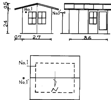
Fig. 1 (b) The dimension of actual House B and the position of pressure measuring points.
