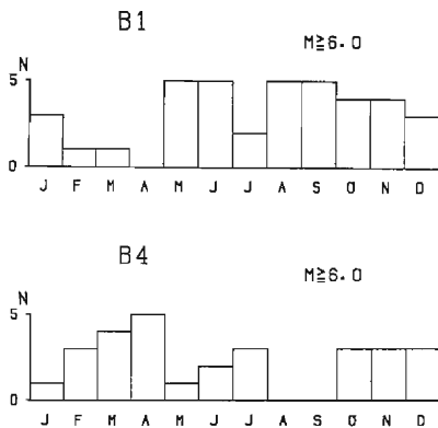
Fig. 11 Monthly distribution of earthquakes ( M \geq 6.0 ) in the B1 and B4 areas.
