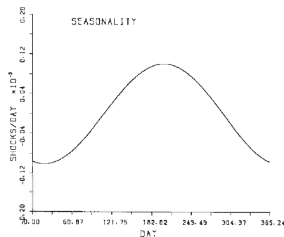
Fig. 58 Seasonal components of the best fitting model of historical earthquakes ( M \geq 7.0 ) in the rectangular area from 110^\circ\text{E} to 120^\circ\text{E} and from 30^\circ\text{N} to 40^\circ\text{N} .
