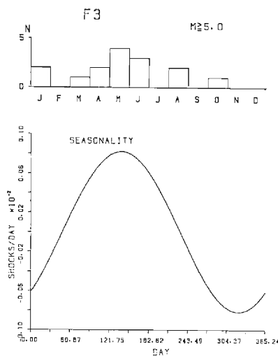
Fig. 28 Monthly distribution of earthquakes ( M \geq 5.0 ) and seasonal components of the best fitting model of inland earthquakes in the north part of the South New Zealand (F3).
