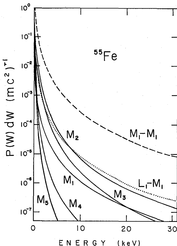
Fig. 1. The ejected electron spectra from M subshells during electron capture decay of ^{55}\text{Fe} . The solid curves represent the M_i -shell spectra in K capture. The dotted curve indicates the M_1 -shell spectrum in L_1 capture and the dashed curve shows that in M_1 capture.
