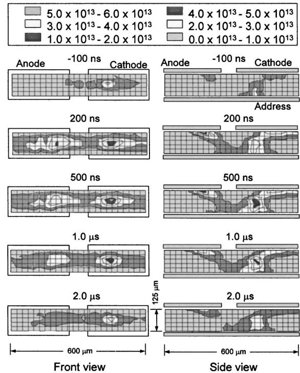
FIG. 3. Temporal sequence of contour diagram of \text{Xe}^*(1s_5) atom density (in units of \text{cm}^{-3} ) at an address pulse voltage of V_a = 60 V viewed from front (left column) and side (right column).
