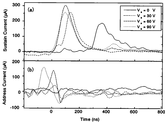
FIG. 4. Wave forms of (a) sustain electrode current I_s and (b) address electrode current I_a measured at address voltages of V_a=0, 30, 60 , and 90 V.
