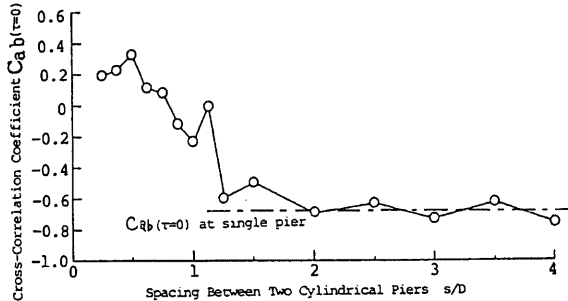
Fig. 12 Relation between the value of C_{ab}(\tau=0) and spacing ratio s/D
