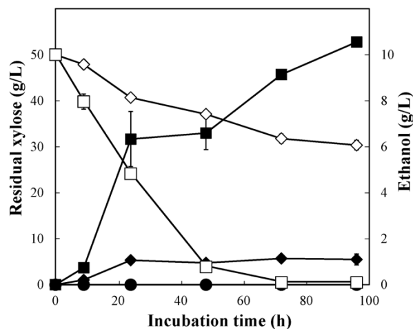
Figure 5. Ethanol production from D-xylose by XylC-displaying yeast strain.
