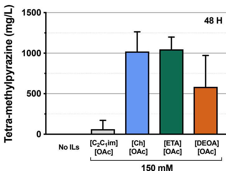
Figure 7. Specific Forms of Ionic Liquids Induce Tetra-methylpyrazine Production in C. glutamicum .
