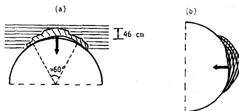
Fig. 13. Tunnel instability occasionally encountered: (a) falling off at the roof of tunnel excavated in a high horizontal stress field (after Lo and Morton 17) ) and (b) rock burst at the side wall.
