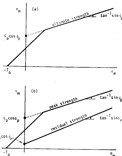
Fig. 4. The modified Mohr-Coulomb criterion employed in the analysis for (a) elasto-plastic material and (b) strain softening material.
