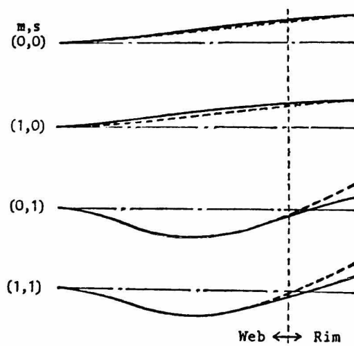
Fig. 3-12 Displacement curves in the radial direction of the web wheel.
