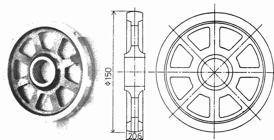
Fig. 7-1 Spoke wheel.
