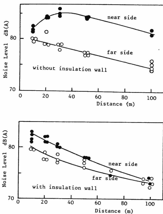
Fig. 2-3 Relation between the noise level and the distance from the track.
