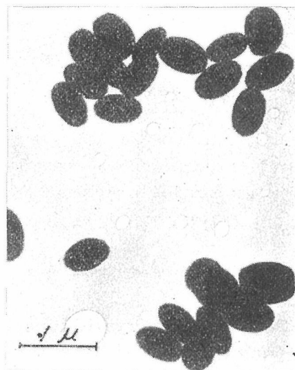
Fig. 2. \text{BaSO}_4 precipitate from Ba-EDTA and \text{H}_2\text{SO}_4 by heating. (b) After completion of precipitation. ( \times 15,000 )
