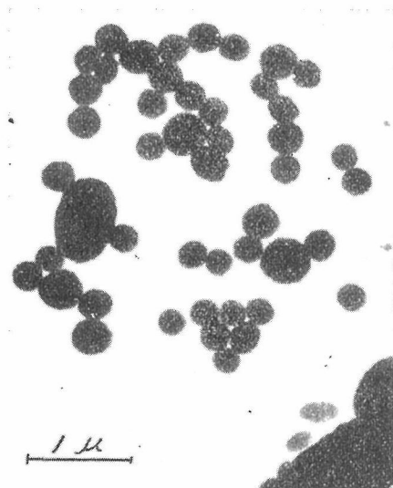
Fig. 1. \text{BaSO}_4 precipitate from Ba-EDTA and \text{H}_2\text{SO}_4 by heating. (a) Initial stage of precipitation. ( \times 15,000 )
