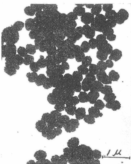
Fig. 4. \text{BaSO}_4 precipitate from Ba-EDTA and (\text{NH}_4)_2\text{S}_2\text{O}_8 by heating. ( \times 12,000 )
