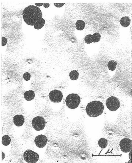
Fig. 3. \text{BaSO}_4 precipitate from Ba-EDTA and \text{H}_2\text{SO}_4 by addition of Zn ion. ( \times 12,000 )
