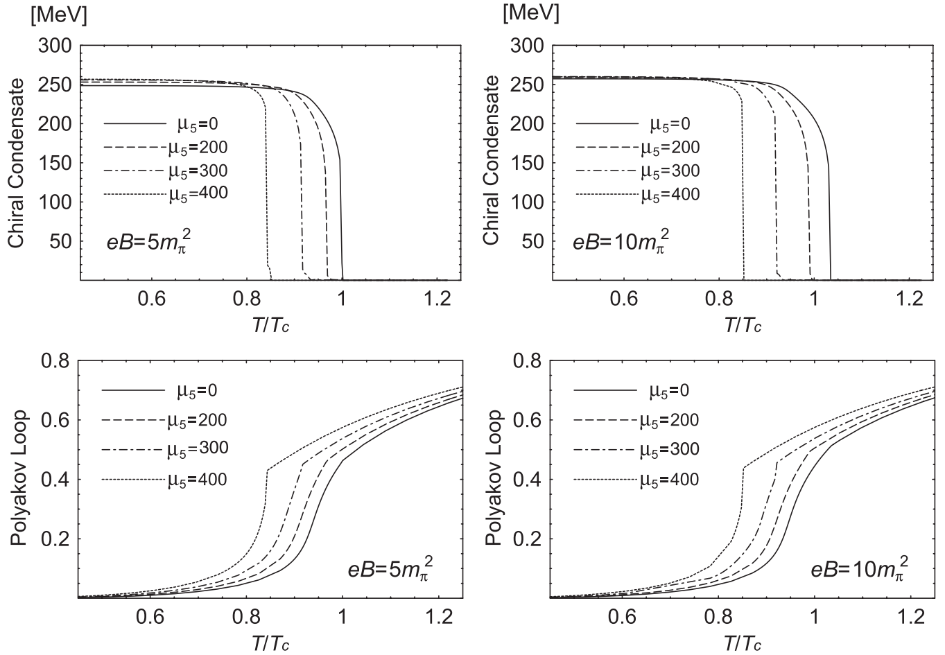
FIG. 2. Absolute value of the chiral condensate |\langle\bar{u}u\rangle|^{1/3} (upper panel) and expectation value of the Polyakov loop (lower panel) as a function of T computed at several values of eB (in units of m_\pi^2 ) and \mu_5 (in units of MeV).
