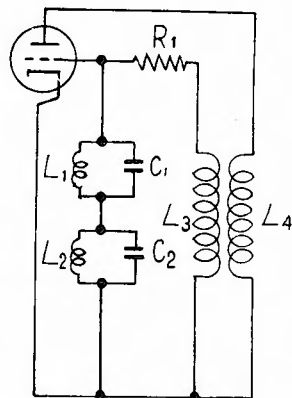
Fig. 1 High frequency current generator
