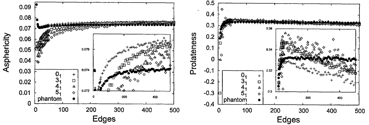
Figure 1: Scaling profiles for the average asphericity (left) and average prolateness (right) of knotted polygons and phantom polygons. The insets provide zoomed-in views, permitting better differentiation between polygons forming the different knot types.
