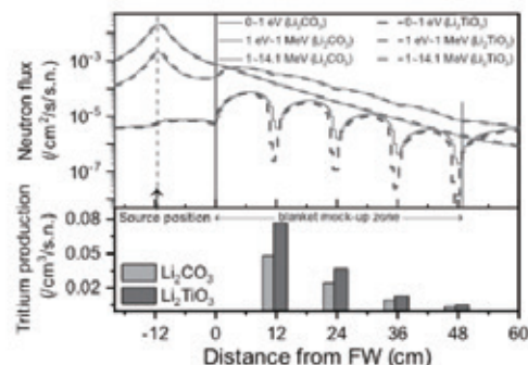
Fig. 2 Neutron fluxes and tritium production rate within a blanket mock-up irradiated with a DT neutron source
