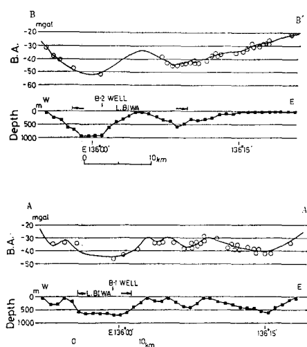
Fig. 12. E-W section along the lines A-A' and B-B' shown in Fig. 11 (after NISHIDA et al. , 1990). B.A. is Bouguer anomaly shown by isogal contours (solid line) and by projections of Bouguer anomaly values at the gravity stations inside the belt zone of 1 km wide from the lines (open circle). Depth is of basement relative to the water level of Lake Biwa at 85 m of altitude. B-1 and B-2 drilling positions are fixed points of basement level in the process of two-dimensional analysis. Assumed density difference between sediments and basement is 0.6 g/cm 3 .
