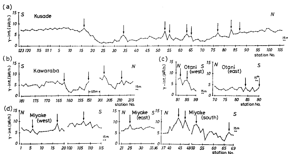
Fig. 5 \gamma -ray profiles of the surveyed lines across the Yagi fault at Sekinomiya (after KATSURA et al. , 1987a). Surveyed sites are shown in Fig. 2. Arrows show the possible positions of fault plane at surface. (a) Kusade, (b) Kawaraba, (c) Otani and (d) Miyake areas.
