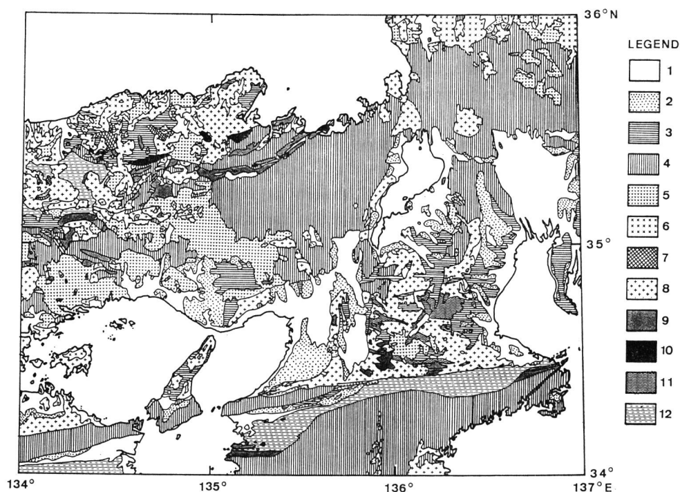
Fig. 42. Geological map of the northern part of Kinki district (modified from YAMADA et al. , 1982). 1: Holocene sediments, 2: Pleistocene sedimentary rocks, 3: Neogene sedimentary rocks, 4: Pre-Neogene sedimentary rocks partly includes basalt, 5: rhyolite and dacite, 6: andesite and basalt, 7: alkali basalt, 8: granitic rocks, 9: gabbro and diorite, 10: ultramafic rocks, 11: low-pressure type metamorphic rocks, 12: high-pressure type metamorphic rocks.
