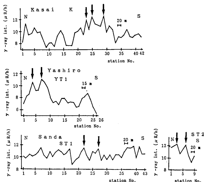
Fig. 18. Examples of \gamma -ray profiles at the surveyed lines across the Sanda-Yamasaki tectonic line (after MOGI et al. , 1985a). Arrows show the possible positions of fault planes at surface. K, YT1 and ST are the N-S survey lines at the Kasai, Yashiro and Sanda areas, respectively, as shown in Fig. 15, Fig. 16(a) and Fig. 17(a).
