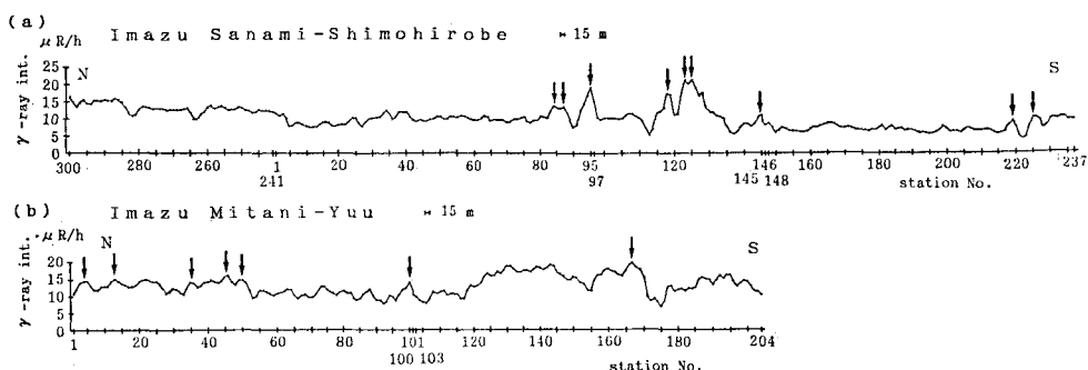
Fig. 35. Examples of \gamma -ray profiles at Imazu. Survey lines are shown in Fig. 34. The data are after smoothing for five points. (a) N-S line from Sanami to Shimo-Hirobe. (b) N-S line from Mitani to Yuu.
