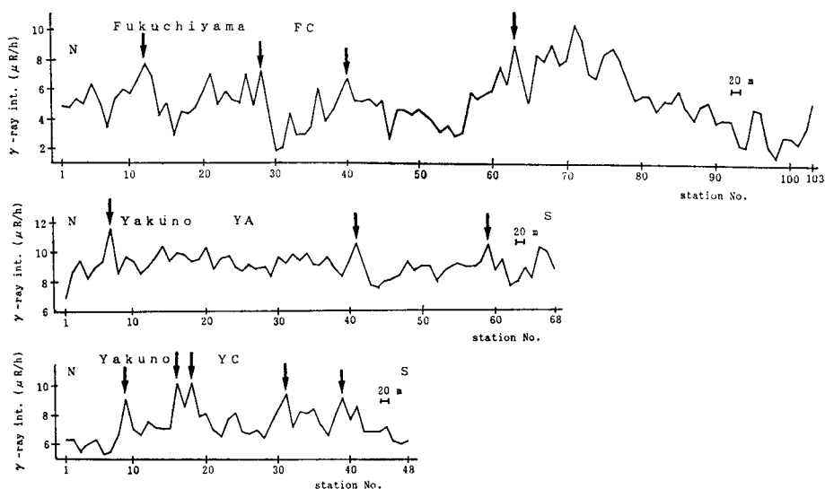
Fig. 22. Examples of N-S \gamma -ray profiles at Fukuchiyama and Yakuno areas (after MOGI et al. , 1985b). Arrows show the possible positions of fault plane at surface. Line name corresponds to Fig. 21.
