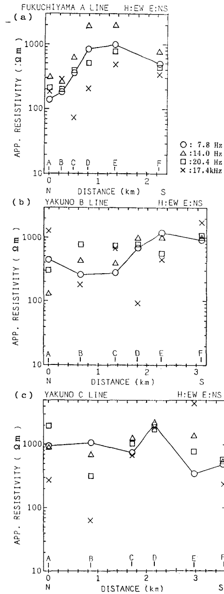
Fig. 23. N-S apparent resistivity profiles of ELF-MT soundings at Fukuchiyama and Yakuno areas (after Mogi et al. , 1985b). Surveyed sites are shown in Fig. 21.
