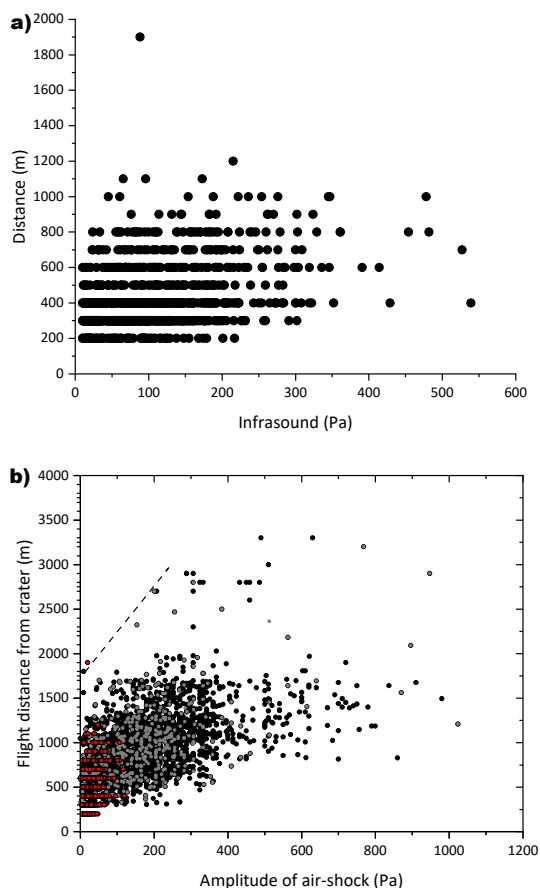
Fig. 4 a) Relationship between amplitude of air-shock (SWA) and flight distance of volcanic bombs ejected by vulcanian eruptions of Suwanosejima volcano. b) Comparison of the relations between Suwanosejima (red) and Sakurajima (black) volcanoes. The amplitude of Suwanosejima was corrected to the value at a distance of 2.7 km (Sakurajima's reference).
