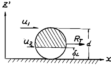
Fig. 2 Schematic drawing of the fluid resistance.
