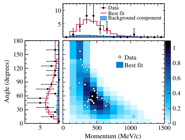
FIG. 3 (color online). The (p_e, \theta_e) distribution for \nu_e candidate events with the MC prediction using the primary method best-fit value of \sin^2 2\theta_{13} = 0.140 (normal hierarchy).
