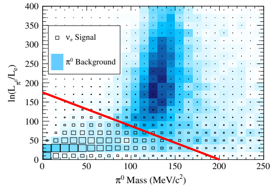
FIG. 2 (color online). The \ln(L_{\pi^0}/L_e) vs m_{\pi^0} distribution is shown for both signal \nu_e -CC events (boxes) and background events containing a \pi^0 (blue scale). The red (gray) line indicates the location of the \pi^0 rejection cut. Events in the upper right corner are rejected.
