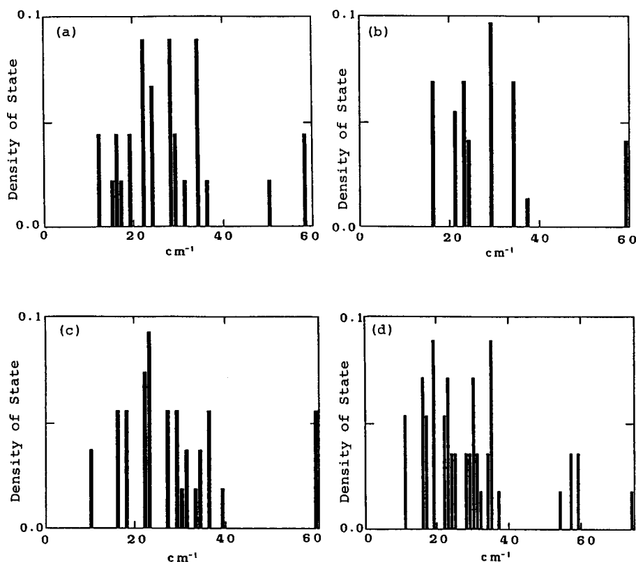
Fig. 10. Normal mode histograms for the lowest potential minimum. (a) \text{Ar}_{12} , (b) \text{Ar}_{13} , (c) \text{Ar}_{14} , (d) \text{Ar}_{19} .
