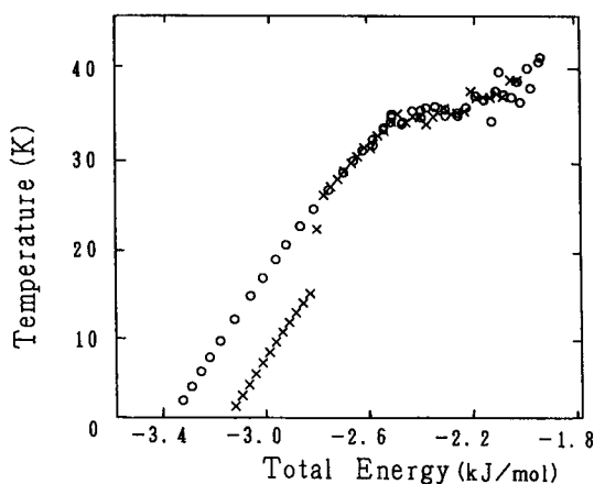
Fig. 7. Caloric curves for \text{Ar}_{13} cluster with LJ potential. Circles are started from icosahedron structure and crosses are started from the second lowest structure.
