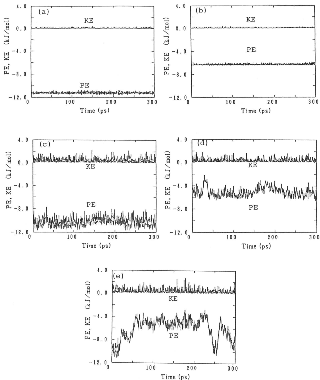
Fig. A2. The kinetic and potential energies of one particle in \text{Ar}_{13} cluster with the LJ potential.
