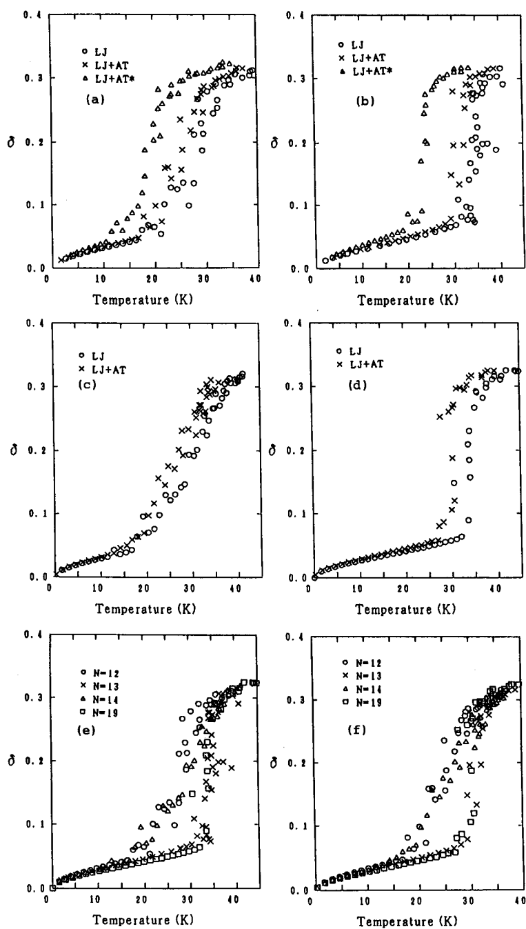
Fig. 5. Relative root-mean-square bond length fluctuations for several cluster sizes. (a) \text{Ar}_{12} (b) \text{Ar}_{13} (c) \text{Ar}_{14} (d) \text{Ar}_{19} (e) LJ clusters (f) LA clusters
