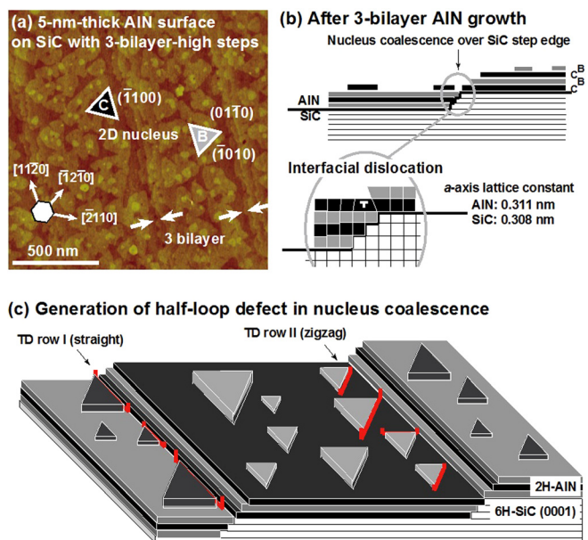
FIG. 4. (a) Surface morphology of 5-nm-thick AlN layer on 6H-SiC (0001) with 3-bilayer-high steps. AlN has a layer-by-layer growth mode. Triangle-shaped 2D nuclei of AlN are observed because of a three-fold symmetry. (b) and (c) Schematic images of generation mechanism of interfacial dislocations in AlN layer on 6H-SiC (0001) with 3-bilayer-high steps. Interfacial dislocations are generated over step edges of the SiC substrate to reduce the tensile strain in nucleus coalescence after 3-bilayer AlN growth.
