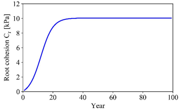
Fig. 6 Time variation of additional cohesion at the slope surface due to root-reinforcement
