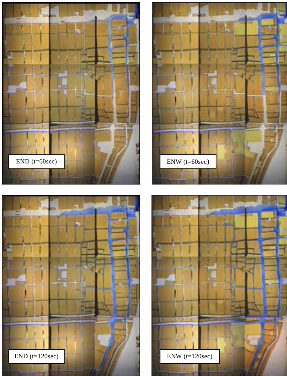
Photo 5 Comparison of flood spreading on dry and wet beds at 60 and 120 second past from the beginning of overflow in the model.
