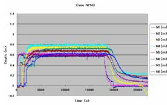
Fig. 18 Water depth of Case NFND in prototype.
