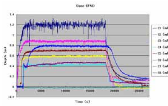
Fig. 14 Water depth of Case EFND in prototype.
