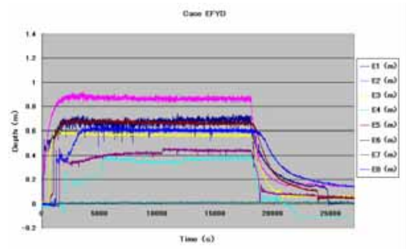
Fig. 15 Water depth of Case EFYD in prototype.
