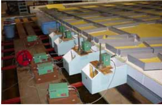
Photo 6 Weirs, level meters, and buckets for discharge measurements. (left : downstream end, right : beneath the model)
