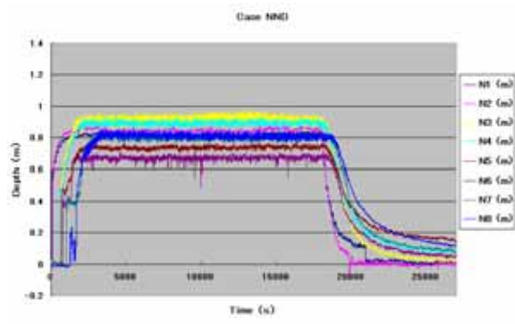
Fig. 16 Water depth of Case NND in prototype.
