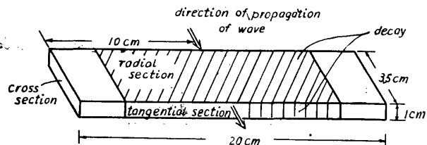
Fig. 5. Specimen tested the dependency of velocity on decay (outer-rot).
