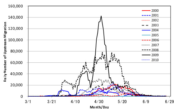
Fig.1 Daily number of upstream migration of sweetfish at Nagara river barrage. 10 days moving averaged data are shown.
