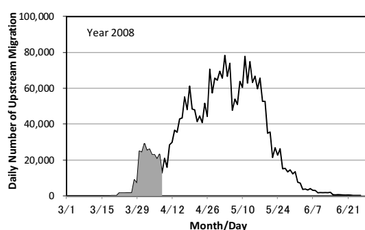
Fig.2 Same as Fig.1, but for the data of 2008 are shown. Shaded area is defined as the first group of upstream migration.
