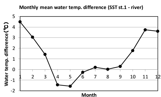
Fig.6 Monthly mean water temperature difference between ocean and river (SST st.1-river). Monthly mean data were calculated from 2001 to 2011.
